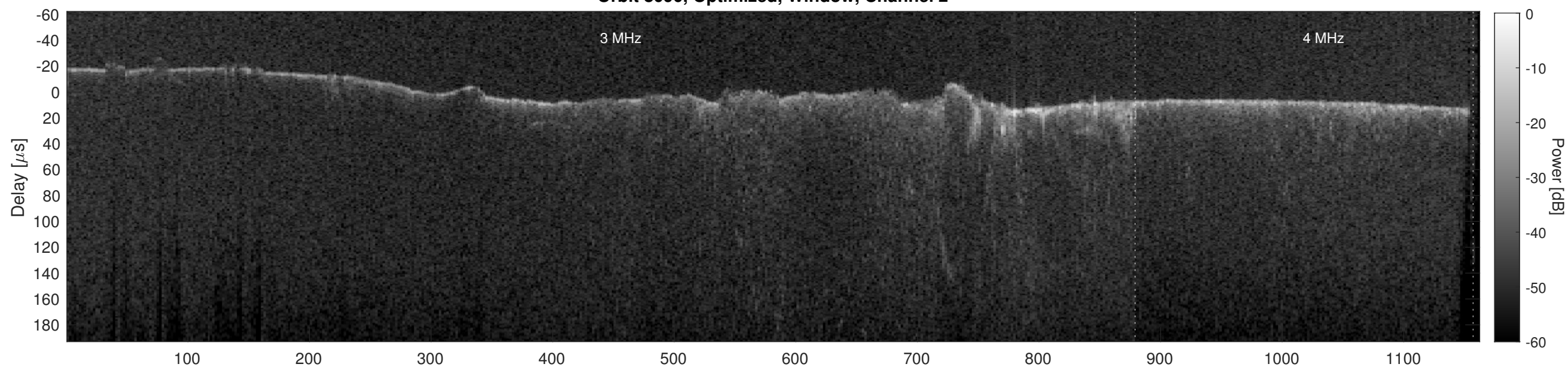
Orbit 8090, Cluttergram
