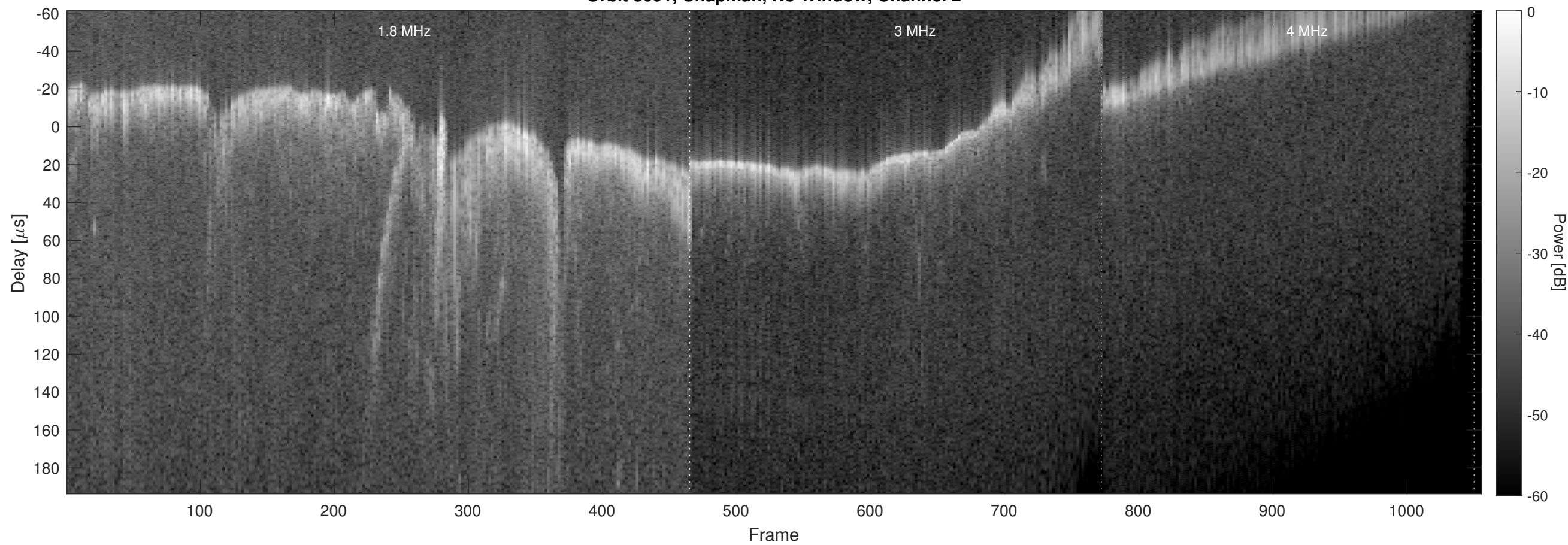
Orbit 8091, Chapman, No Window, Channel 2
