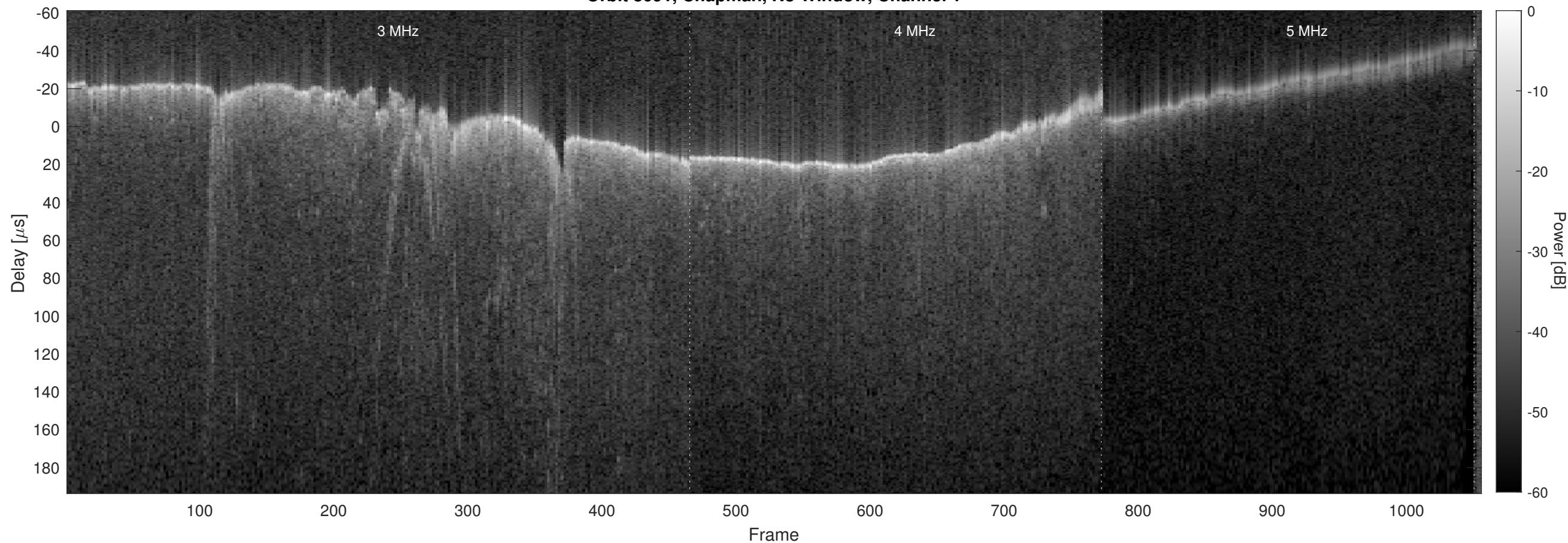
Orbit 8091, Chapman, No Window, Channel 2
