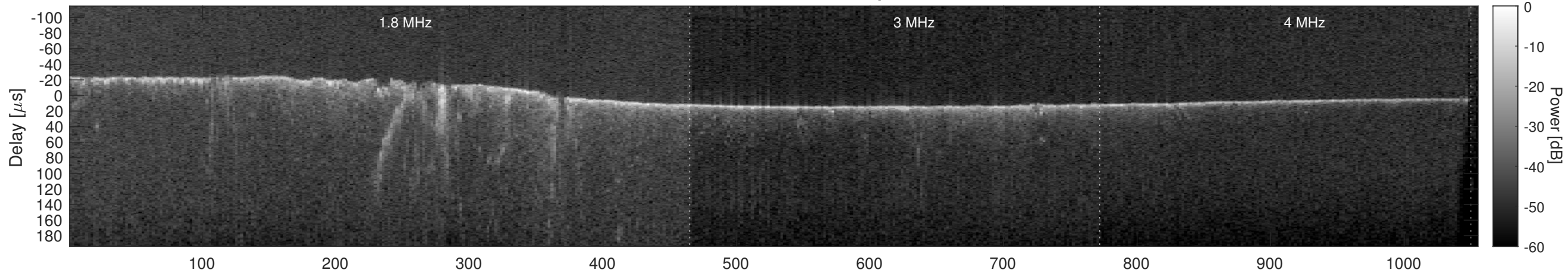
Orbit 8091, Cluttergram
