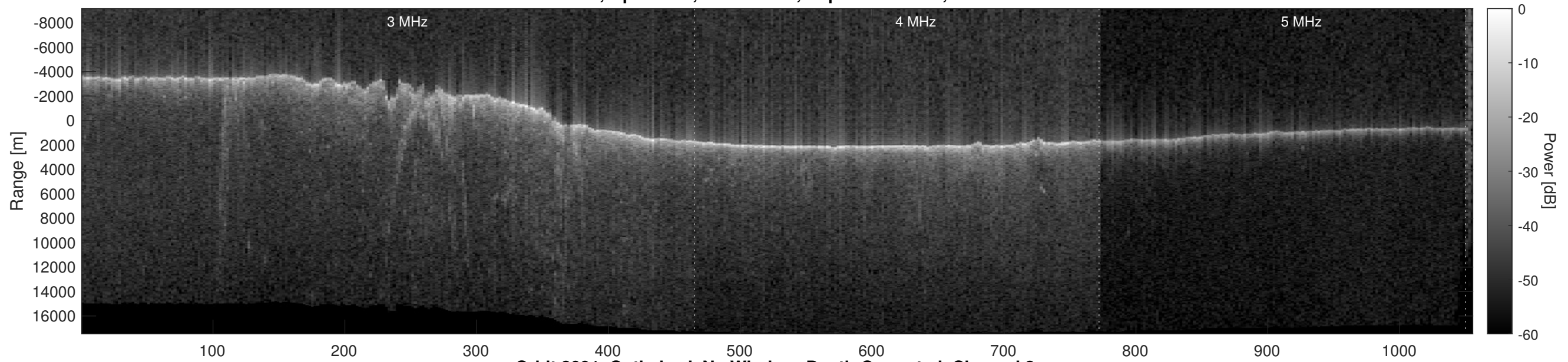
Orbit 8091, Optimized, No Window, Depth-Corrected, Channel 2
