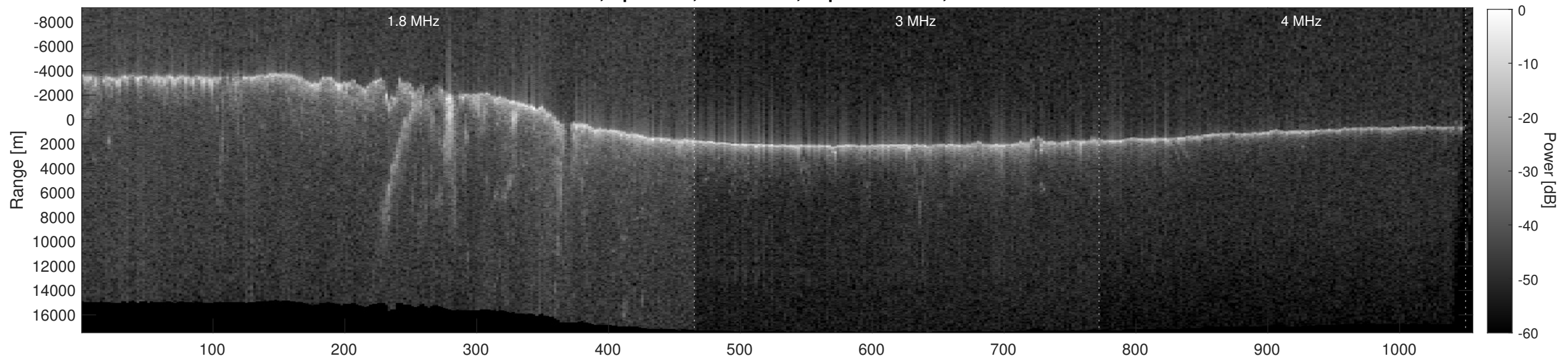
Orbit 8091, Depth-Corrected Cluttergram
