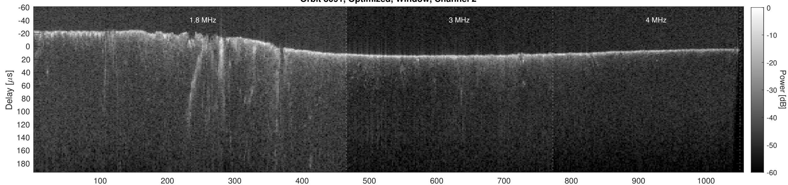
Orbit 8091, Cluttergram
