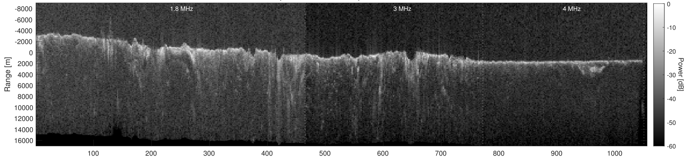
Orbit 8092, Depth-Corrected Cluttergram
