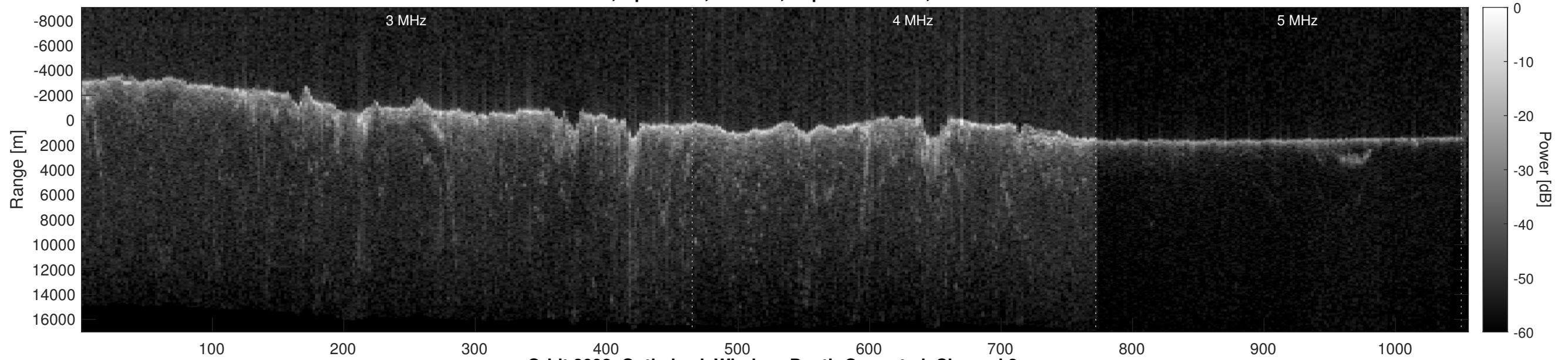
Orbit 8092, Optimized, Window, Depth-Corrected, Channel 2
