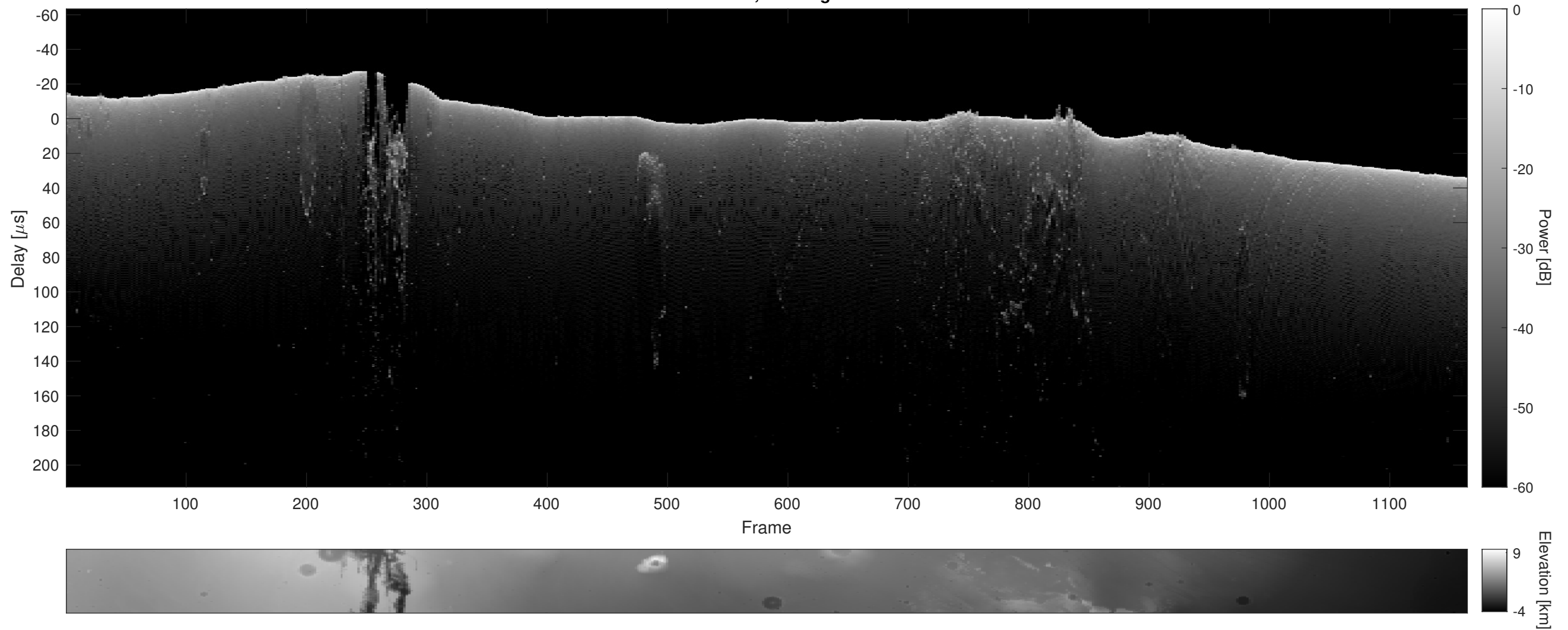
Orbit 8093, Cluttergram
