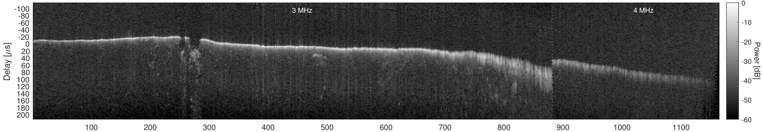
Orbit 8093, Window, Channel 2, Chapman
