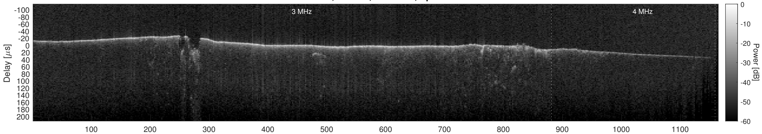
Orbit 8093, Cluttergram
