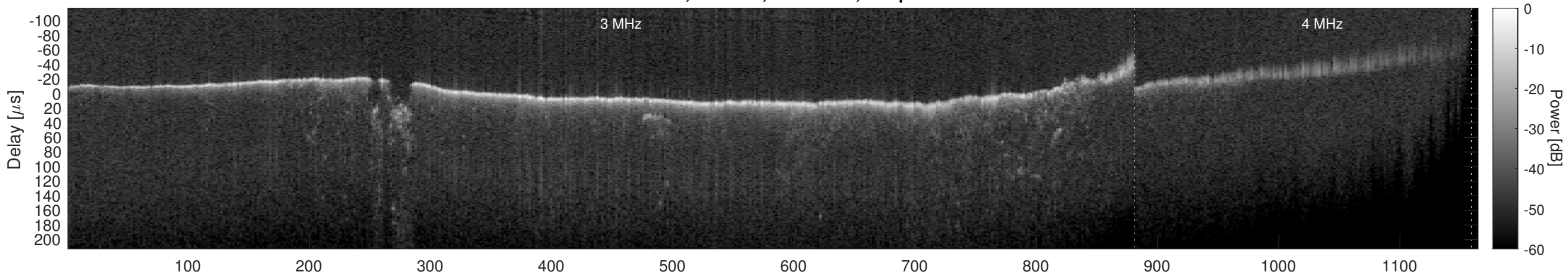
Orbit 8093, Window, Channel 2, Optimized
