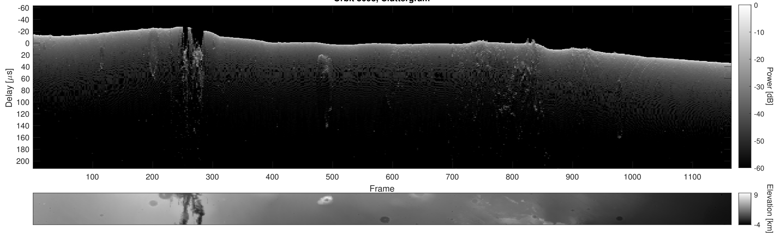
Orbit 8093, Cluttergram
