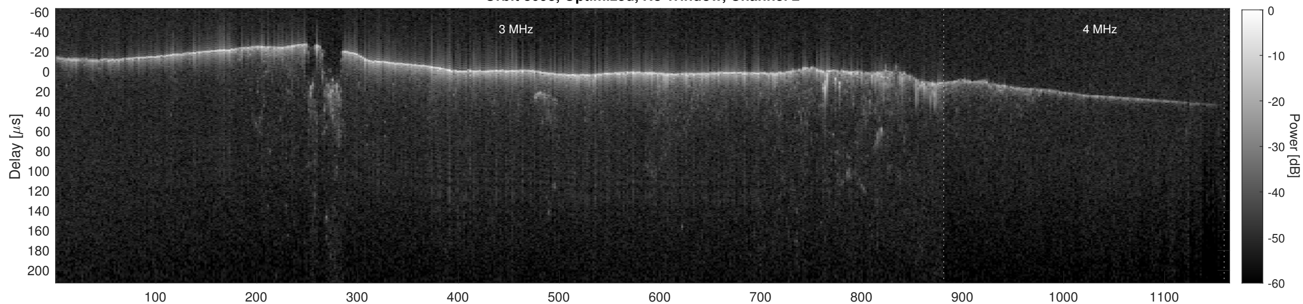
Orbit 8093, Cluttergram
