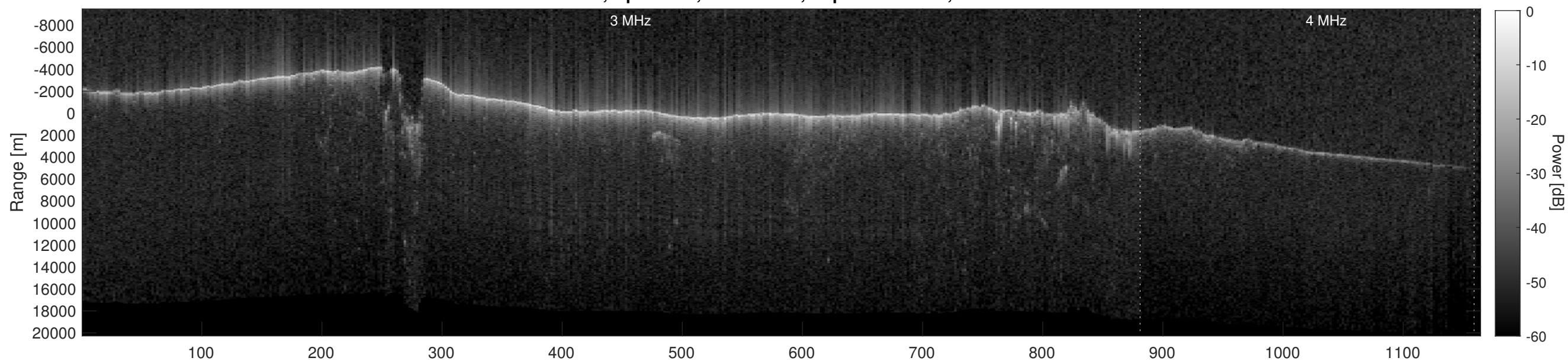
Orbit 8093, Depth-Corrected Cluttergram
