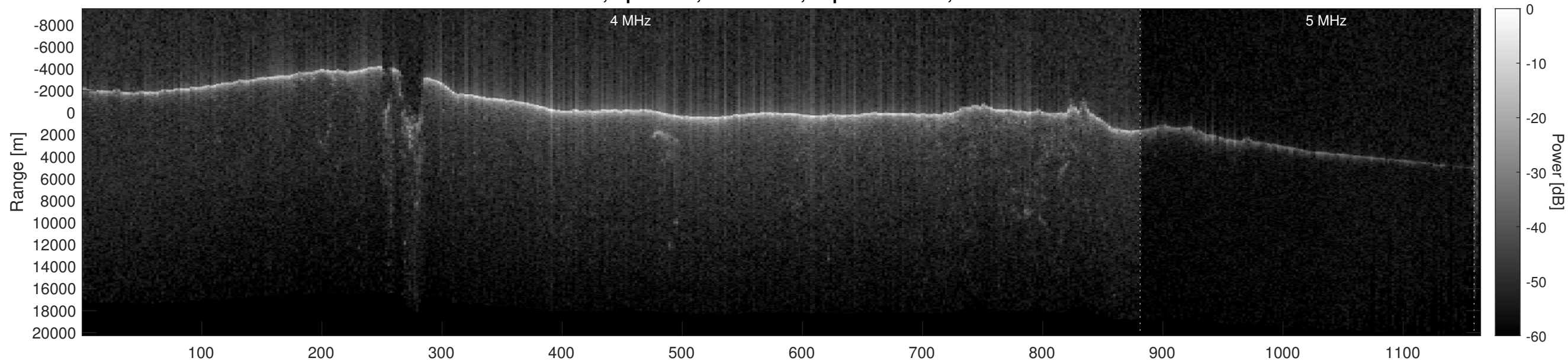
Orbit 8093, Optimized, No Window, Depth-Corrected, Channel 2
