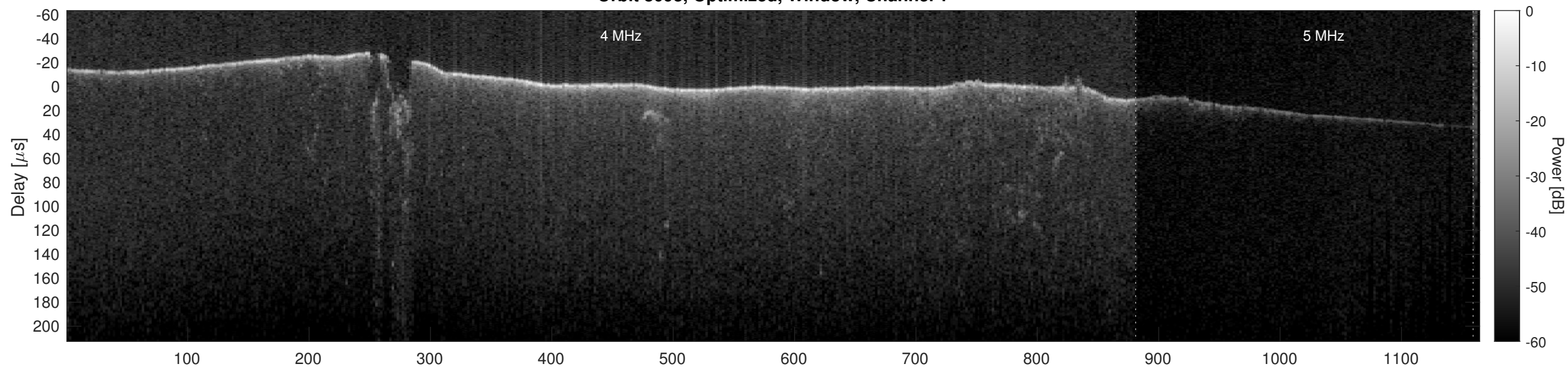
Orbit 8093, Optimized, Window, Channel 2
