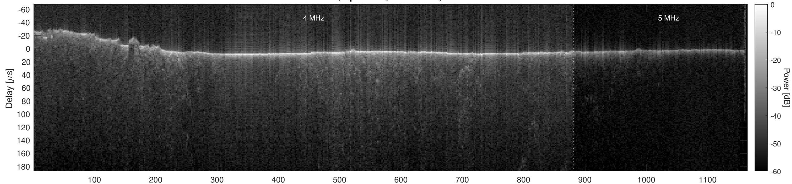
Orbit 8094, Optimized, No Window, Channel 2
