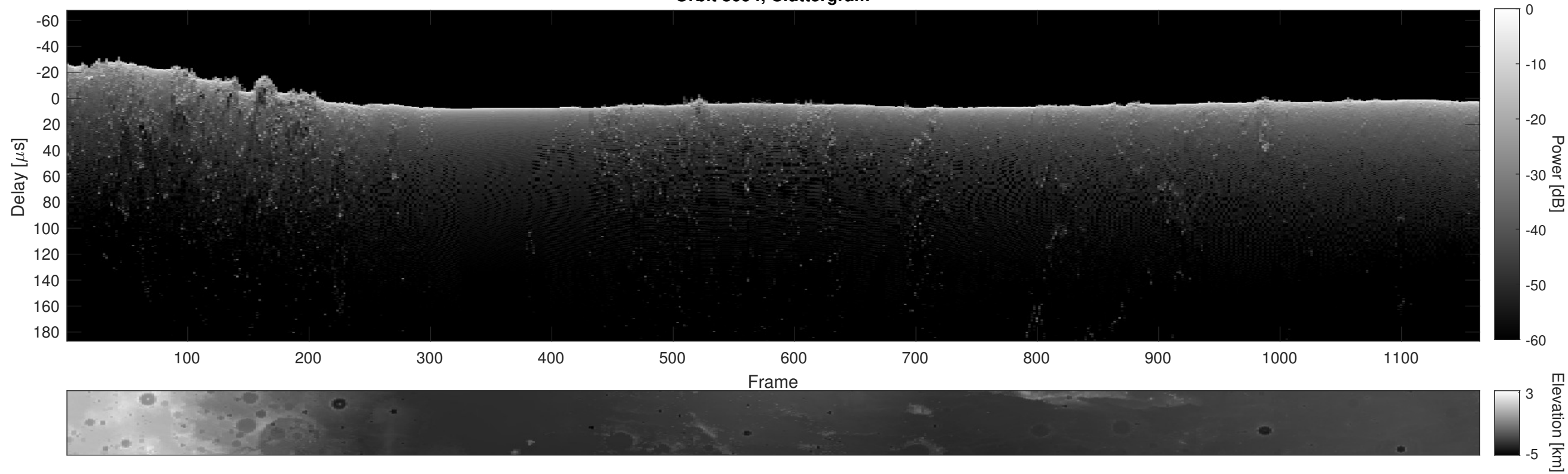
Orbit 8094, Cluttergram
