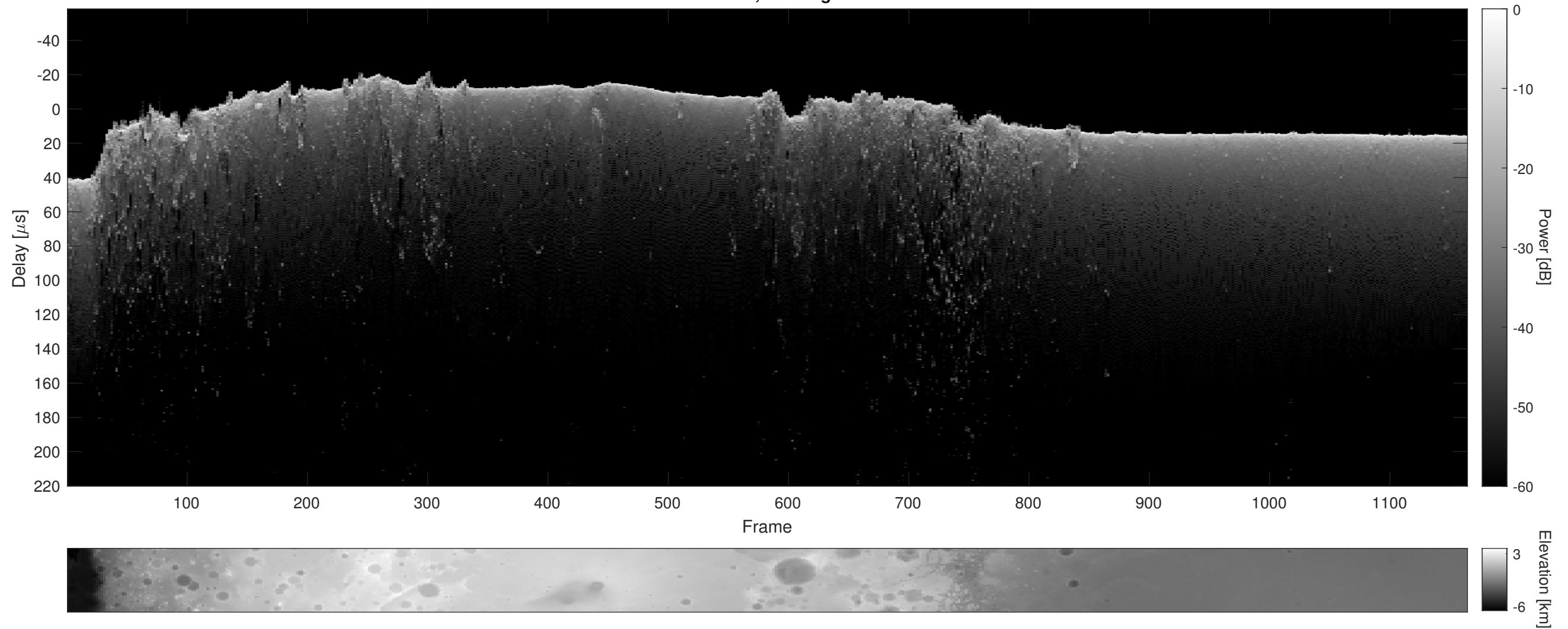
Orbit 8095, Cluttergram
