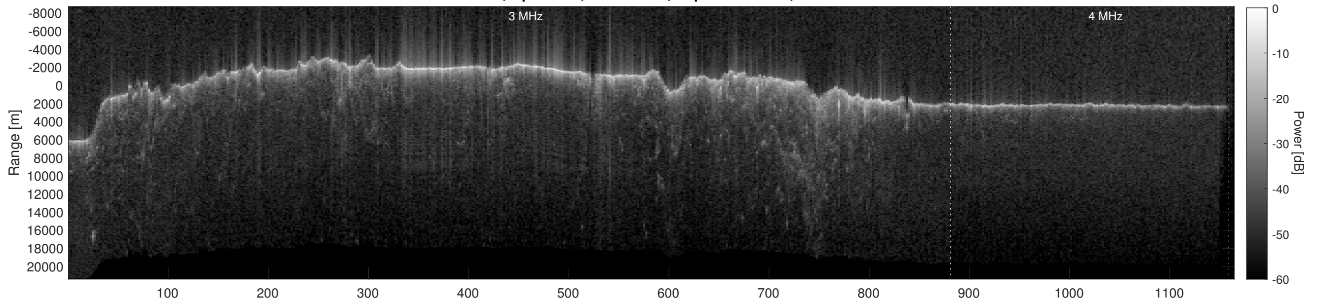
Orbit 8095, Depth-Corrected Cluttergram
