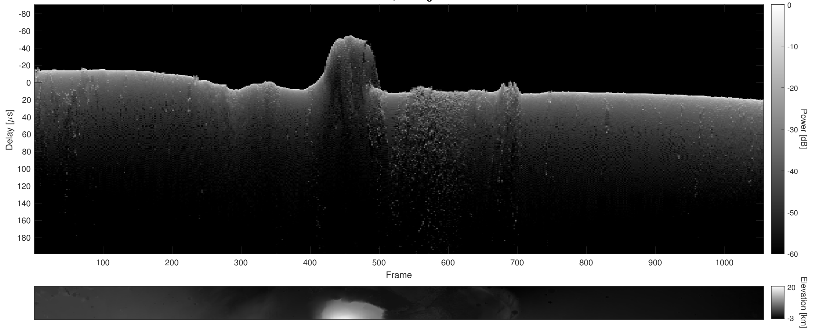
Orbit 8097, Cluttergram
