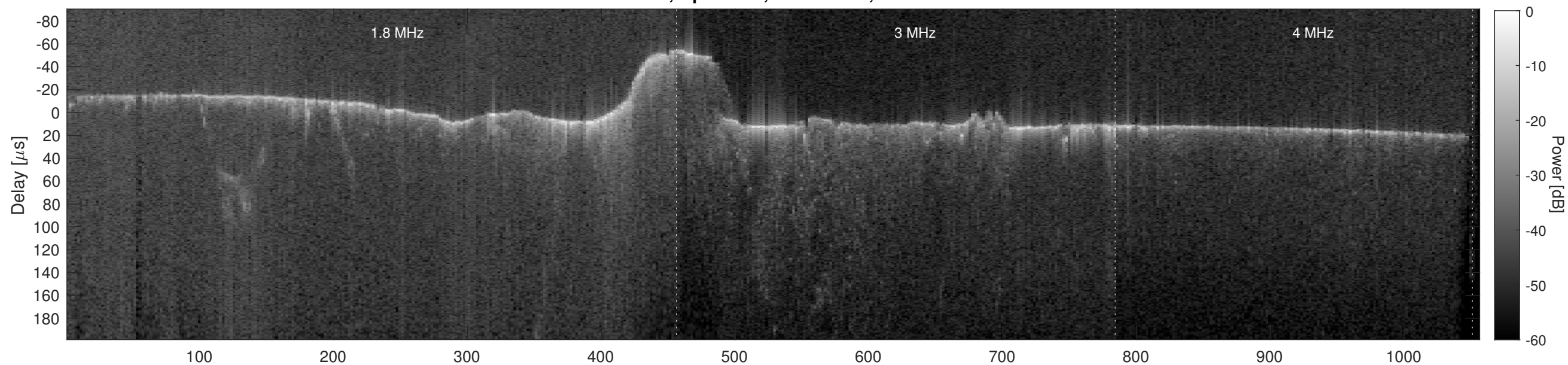
Orbit 8097, Cluttergram
