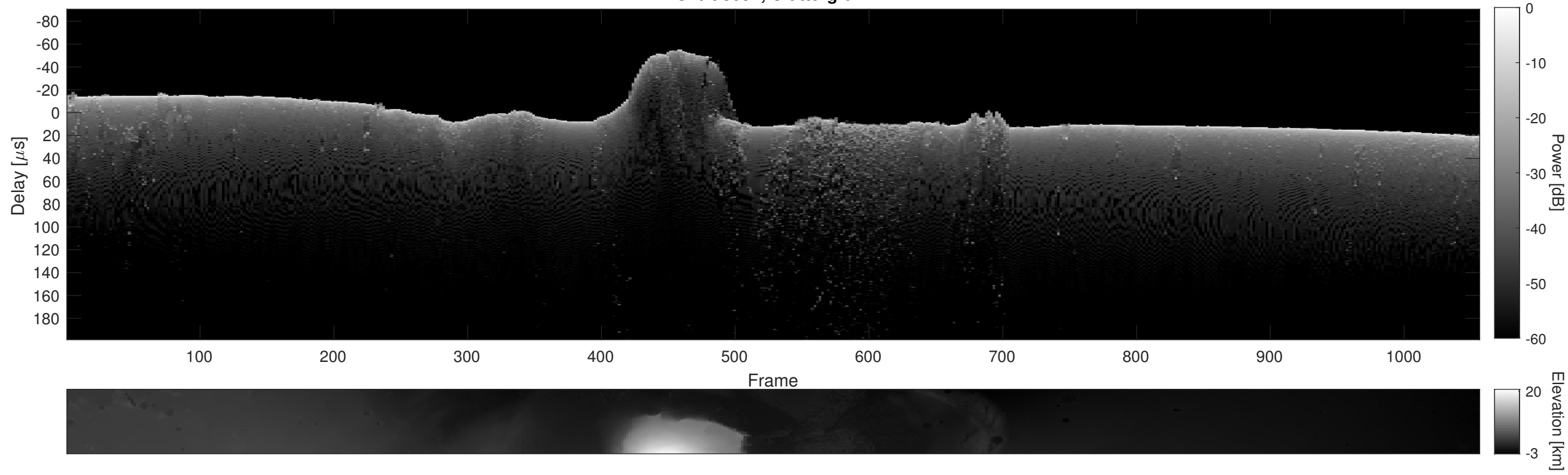
Orbit 8097, Cluttergram
