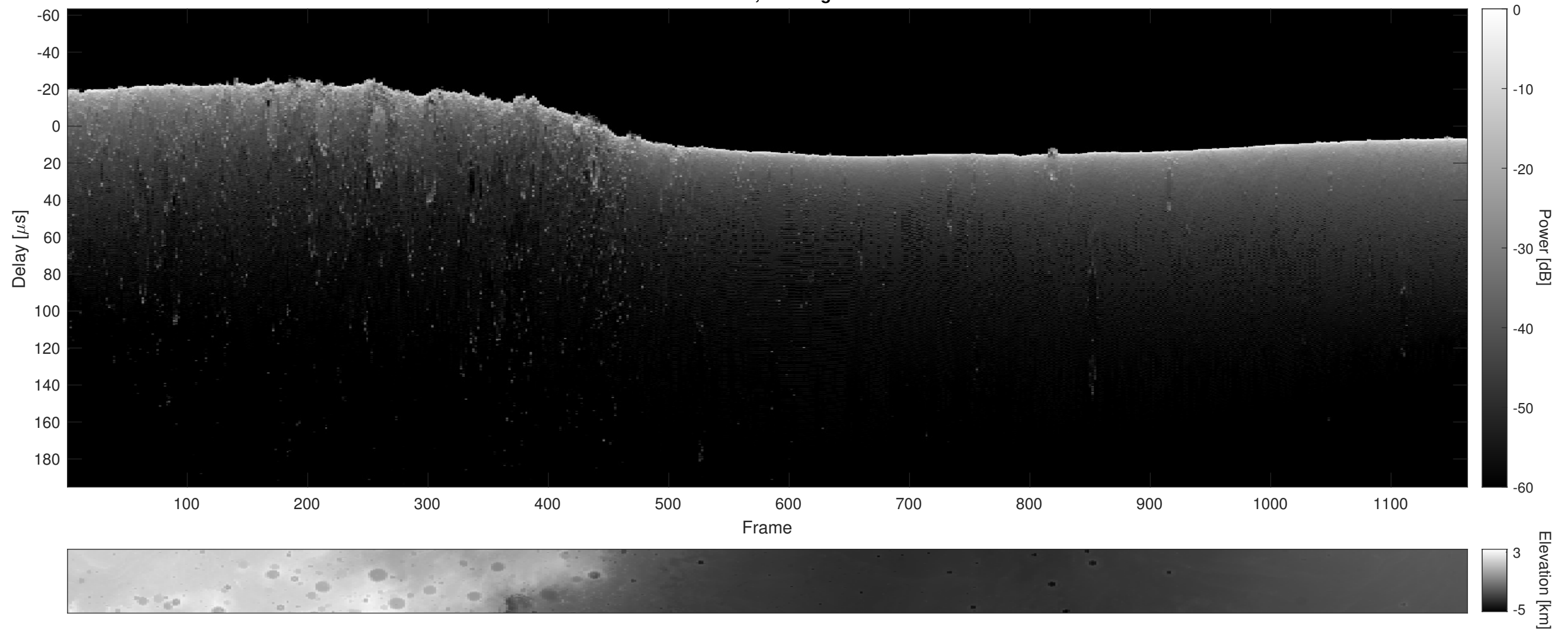
Orbit 8098, Cluttergram
