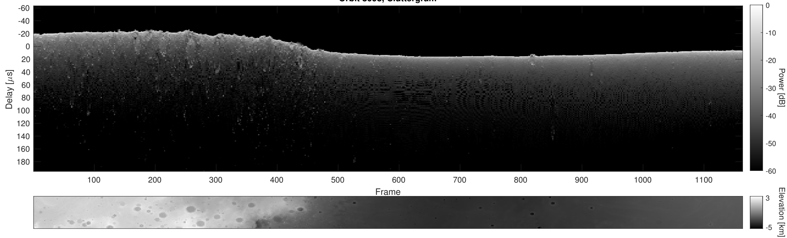
Orbit 8098, Cluttergram
