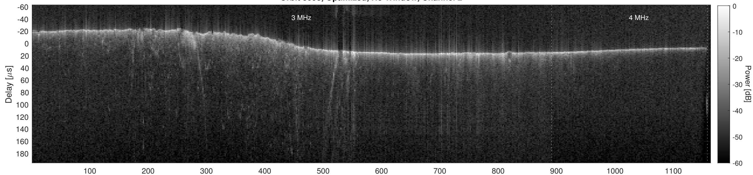
Orbit 8098, Cluttergram
