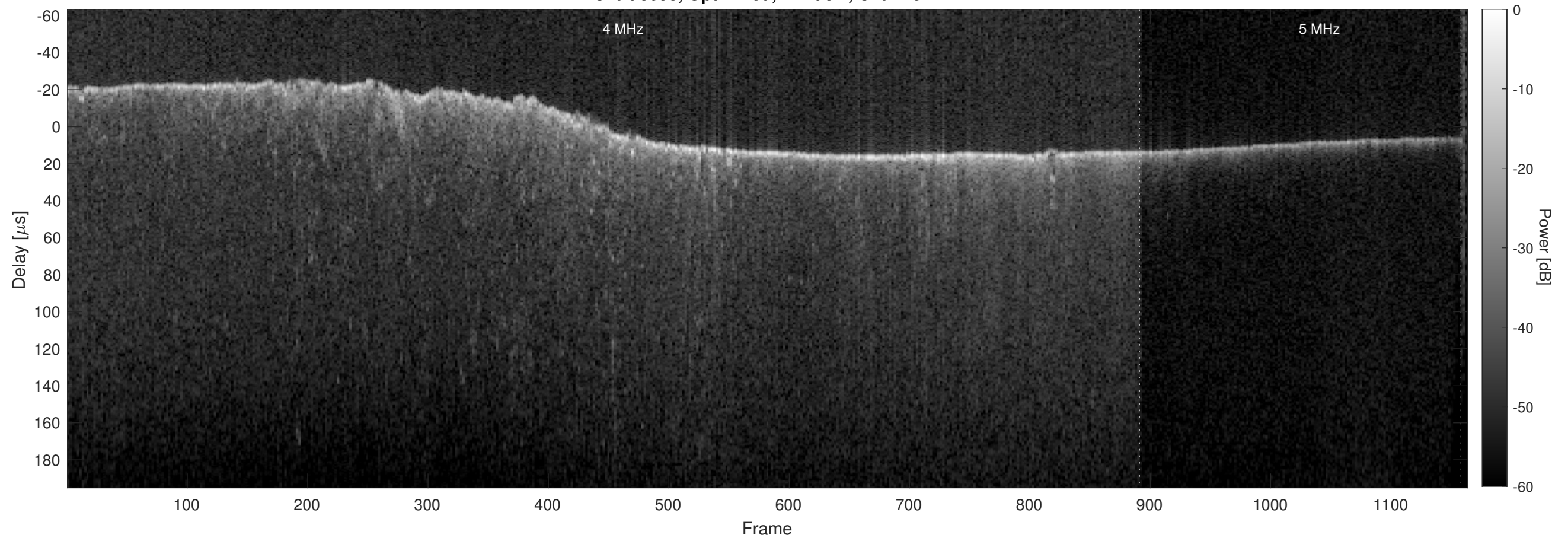
Orbit 8098, Optimized, Window, Channel 2
