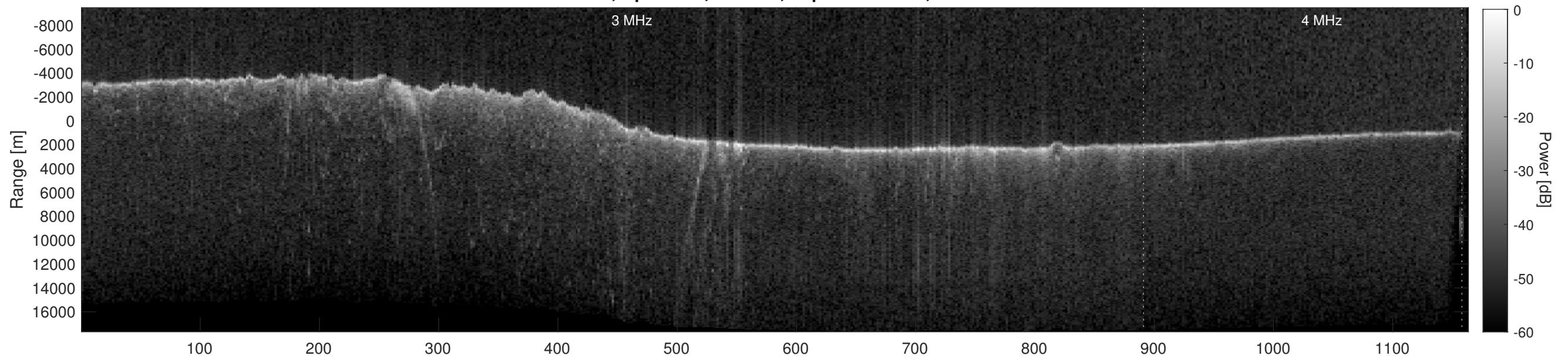
Orbit 8098, Depth-Corrected Cluttergram
