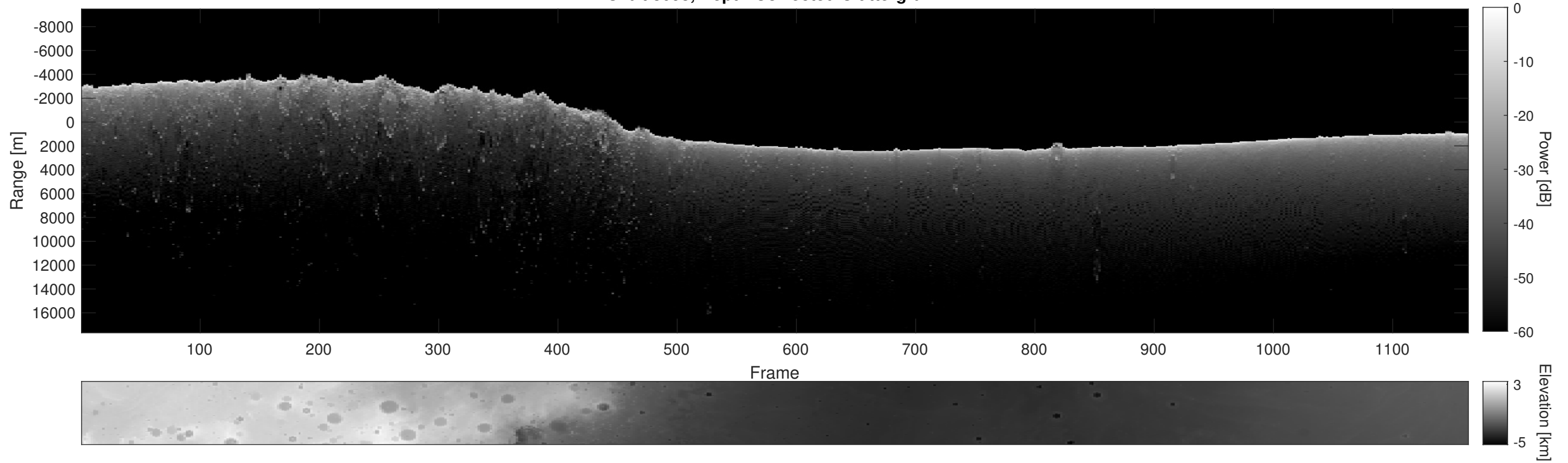
Orbit 8098, Depth-Corrected Cluttergram
