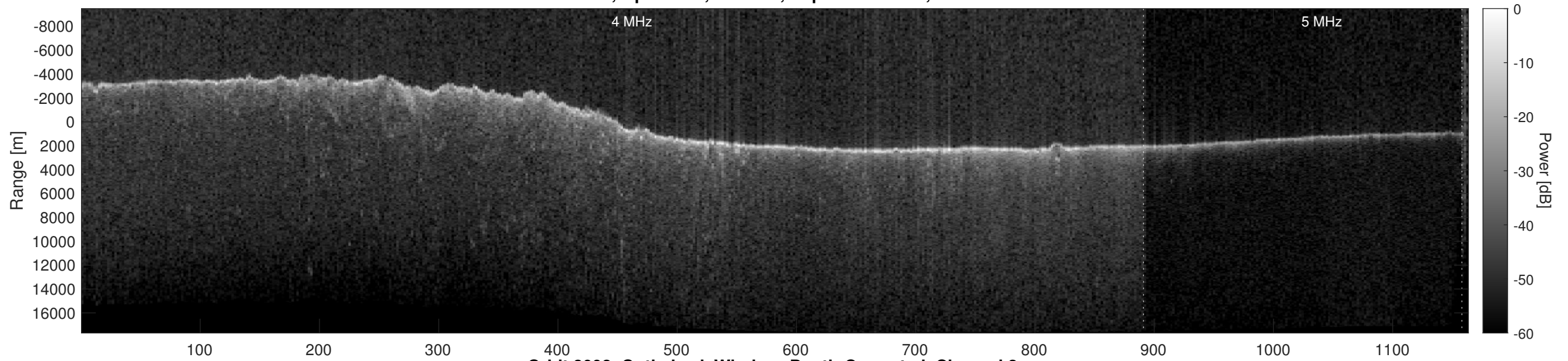
Orbit 8098, Optimized, Window, Depth-Corrected, Channel 2
