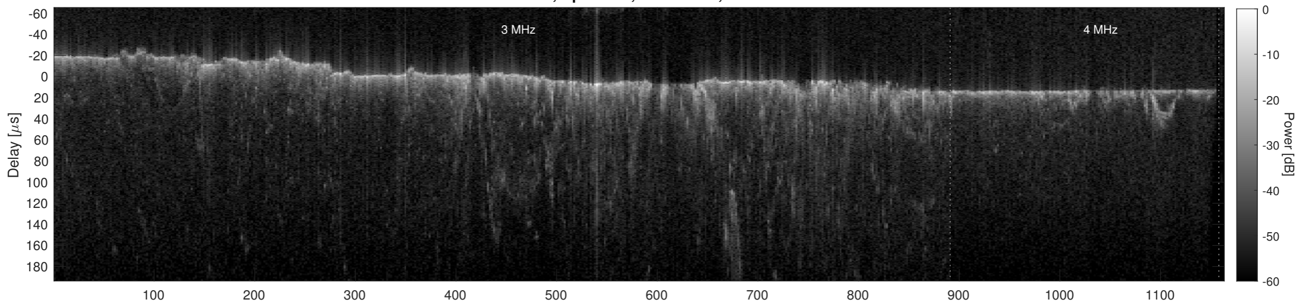
Orbit 8099, Cluttergram
