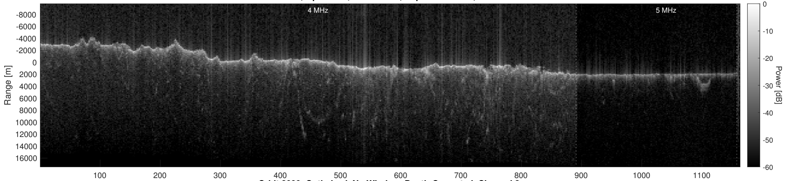
Orbit 8099, Optimized, No Window, Depth-Corrected, Channel 2
