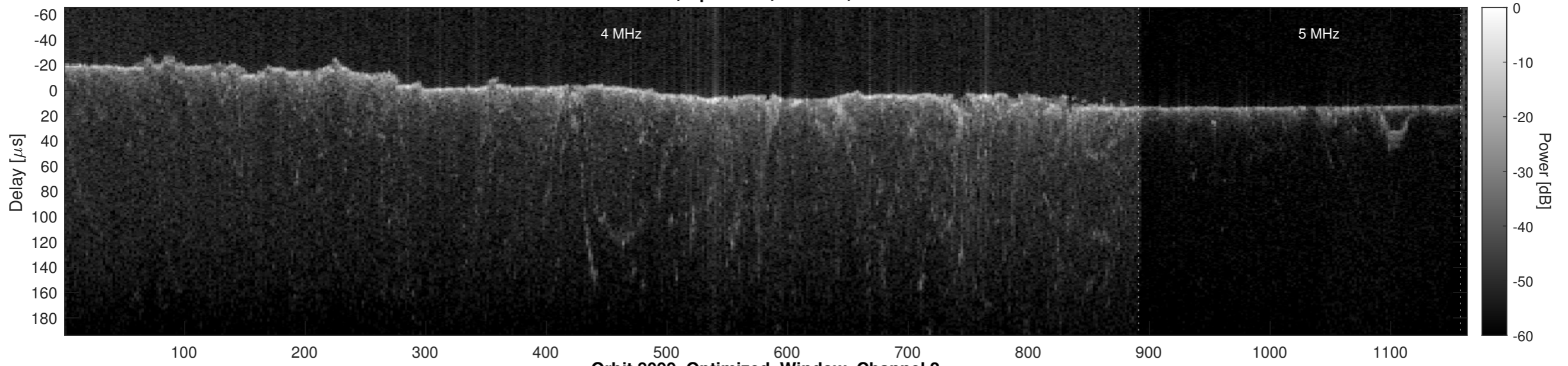
Orbit 8099, Optimized, Window, Channel 2
