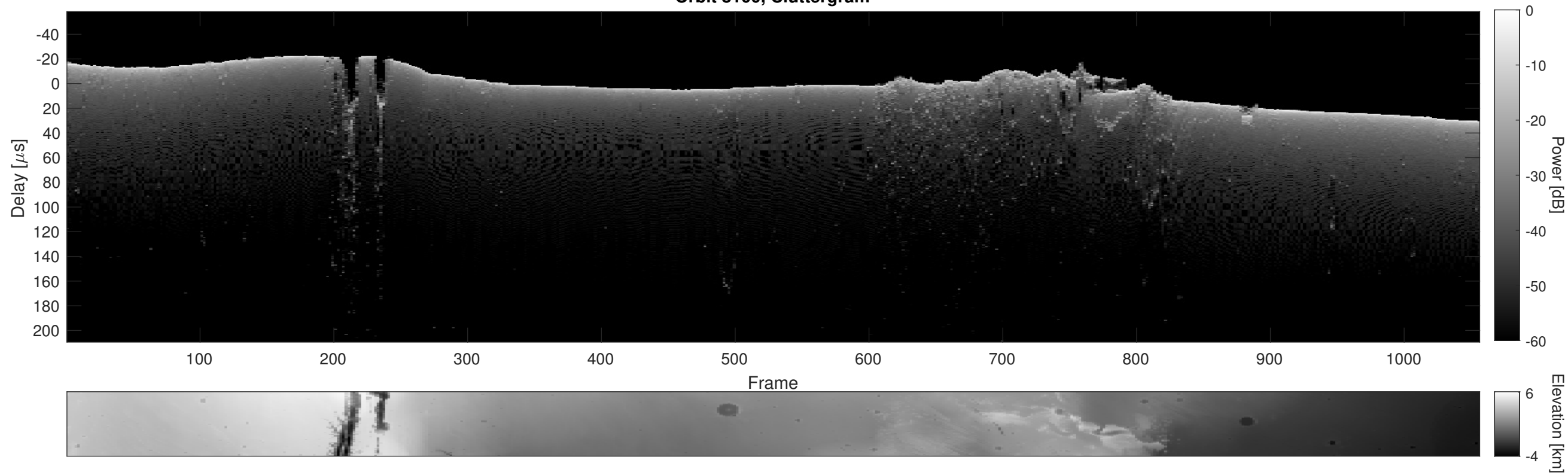
Orbit 8100, Cluttergram
