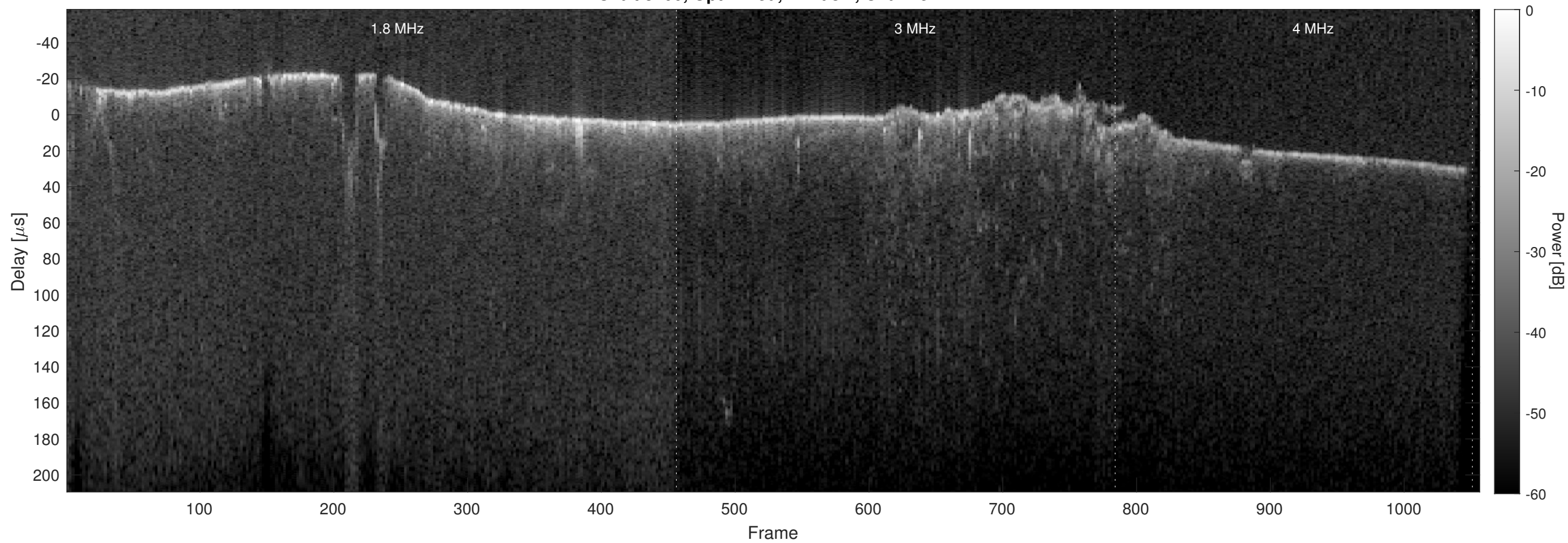
Orbit 8100, Optimized, Window, Channel 2
