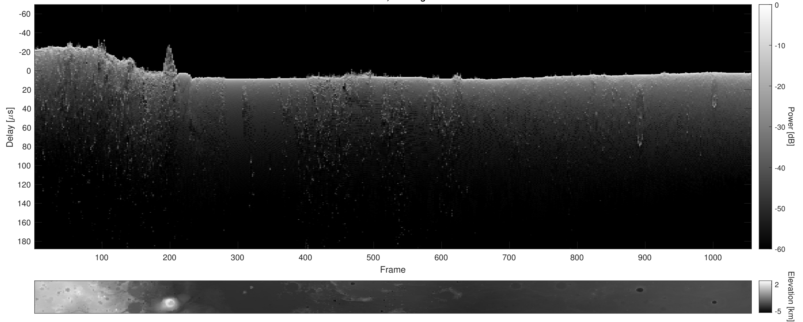
Orbit 8101, Cluttergram
