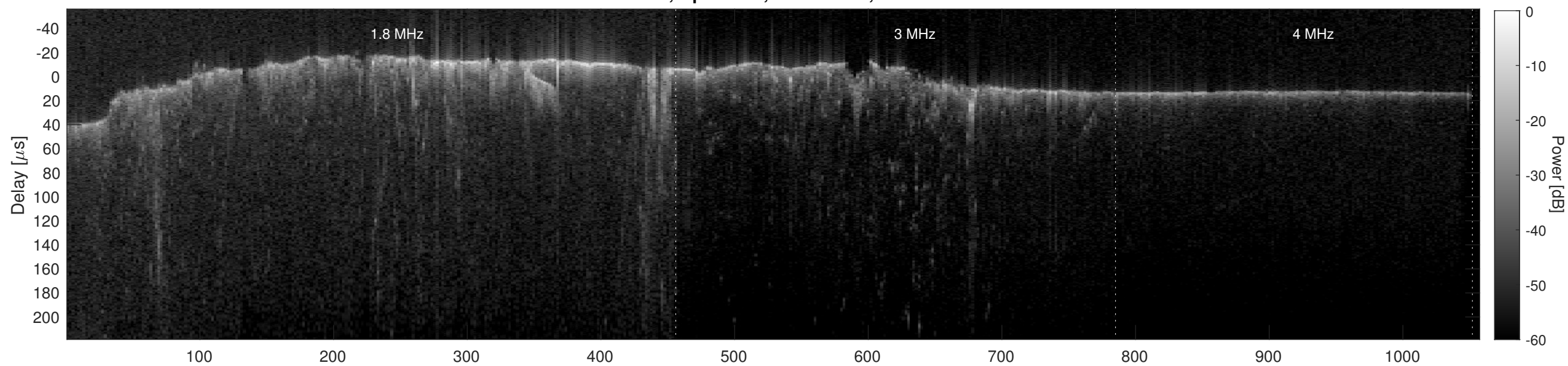
Orbit 8102, Cluttergram
