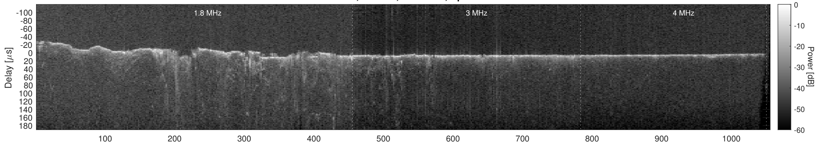
Orbit 8103, Cluttergram
