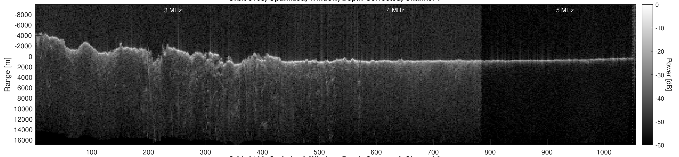
Orbit 8103, Optimized, Window, Depth-Corrected, Channel 2
