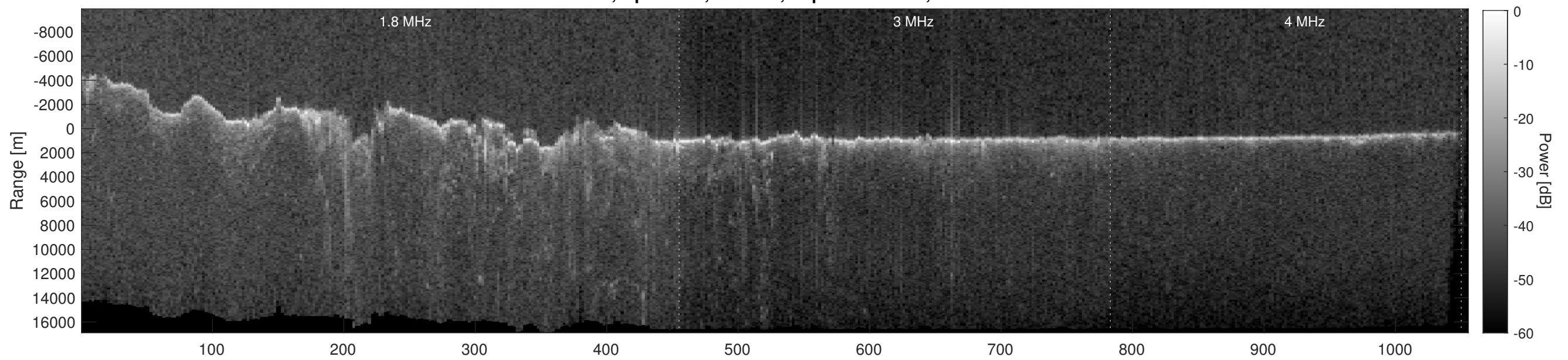
Orbit 8103, Depth-Corrected Cluttergram
