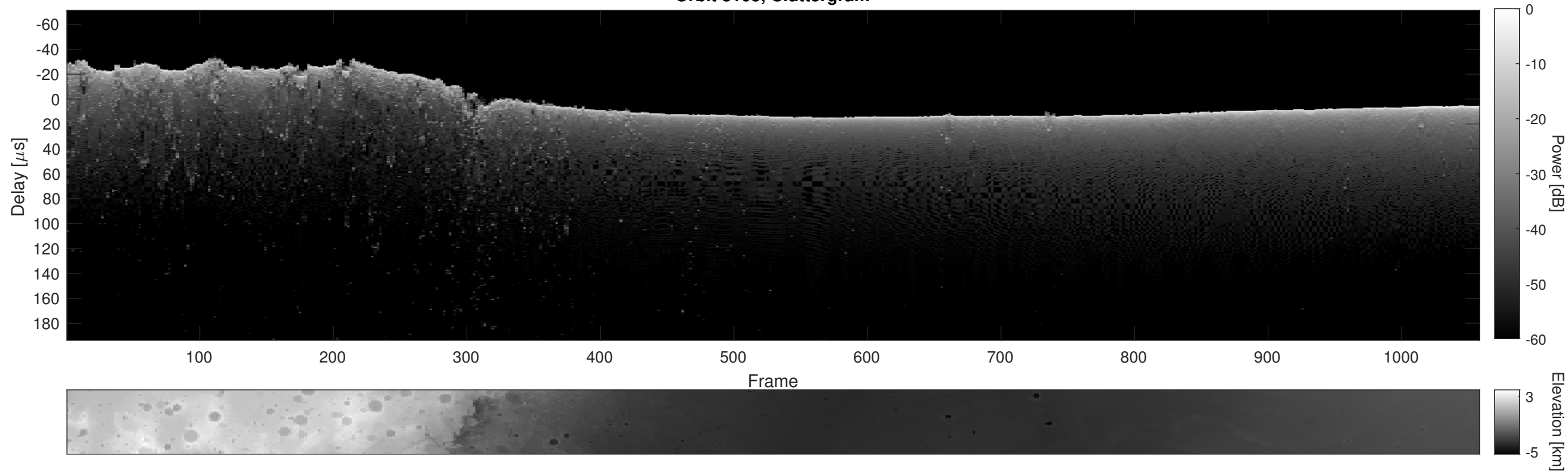
Orbit 8105, Cluttergram
