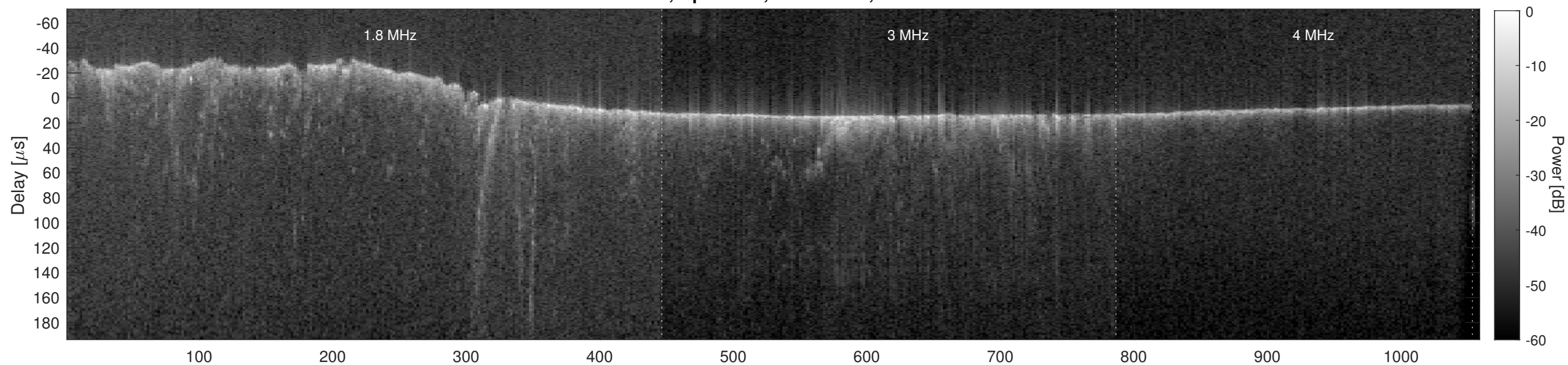
Orbit 8105, Cluttergram
