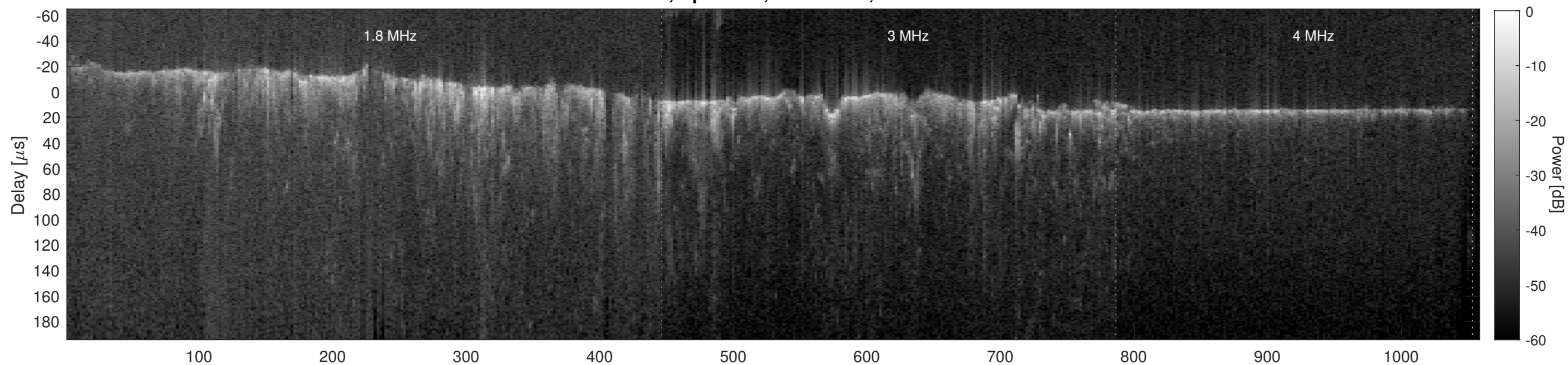
Orbit 8106, Cluttergram
