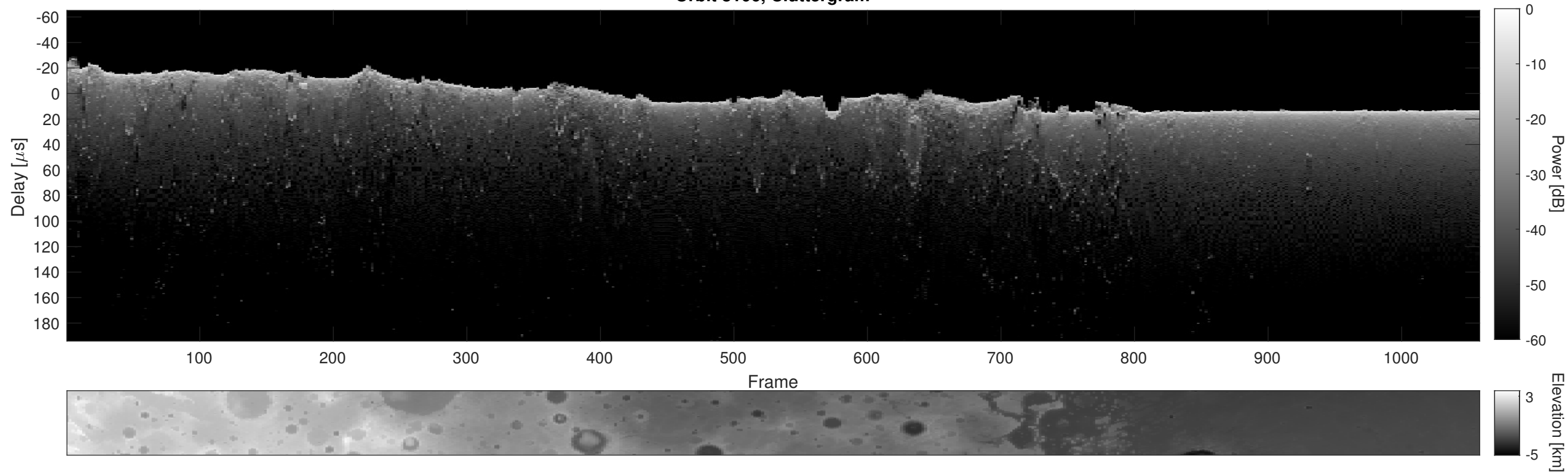
Orbit 8106, Cluttergram
