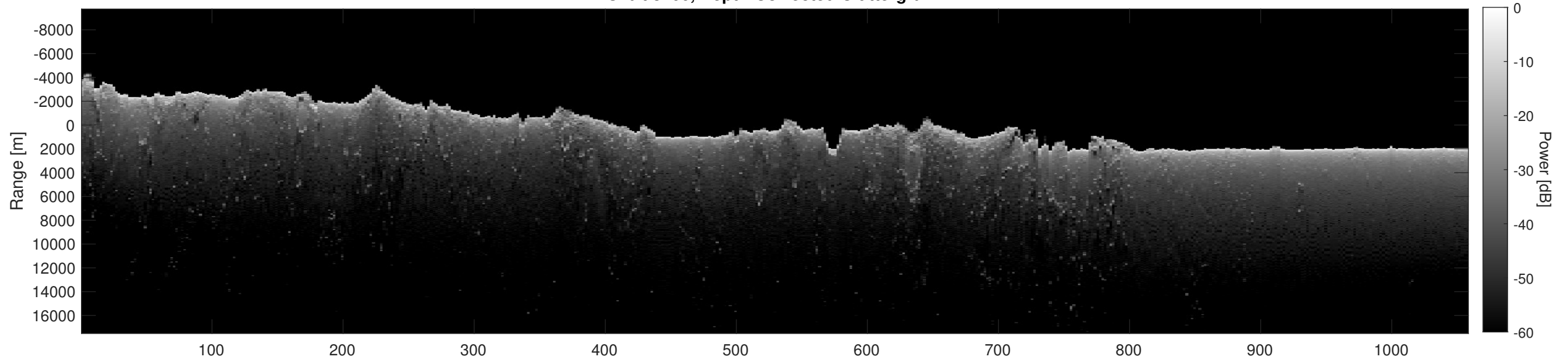
Orbit 8106, Depth-Corrected Cluttergram
