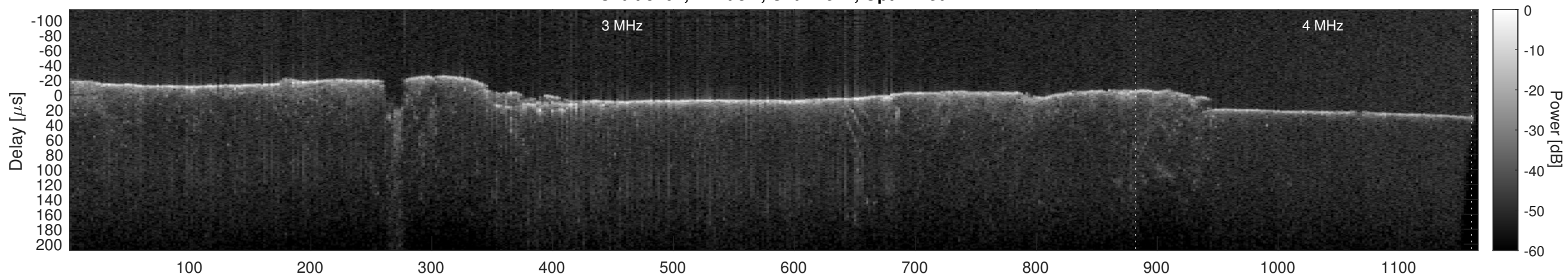
Orbit 8107, Cluttergram
