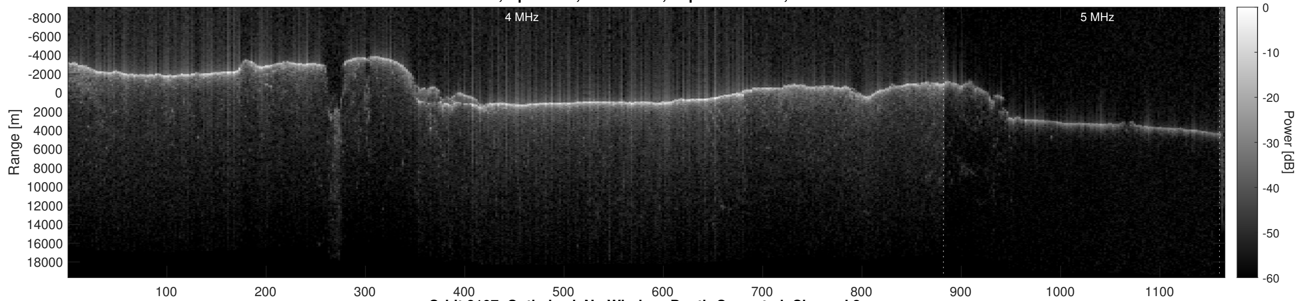
Orbit 8107, Optimized, No Window, Depth-Corrected, Channel 2
