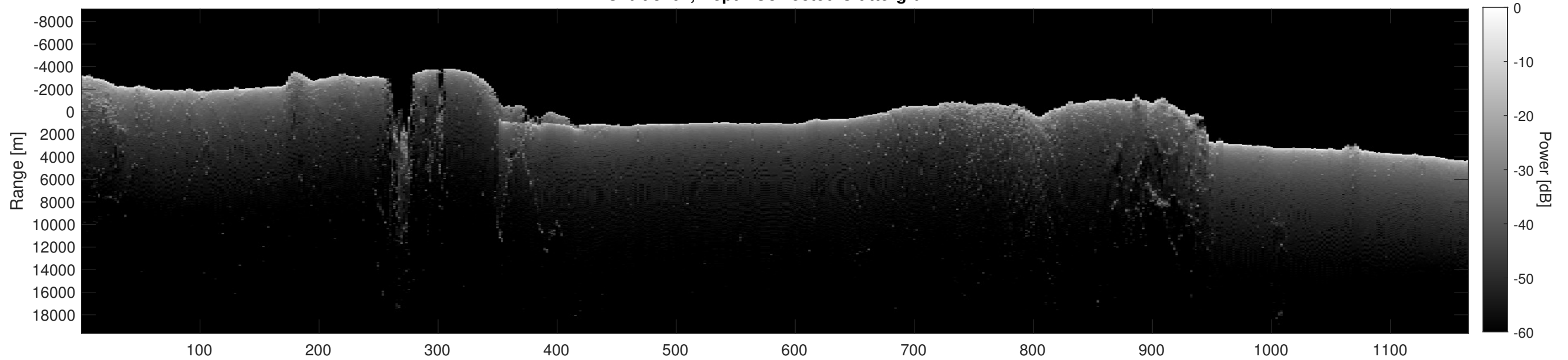
Orbit 8107, Depth-Corrected Cluttergram
