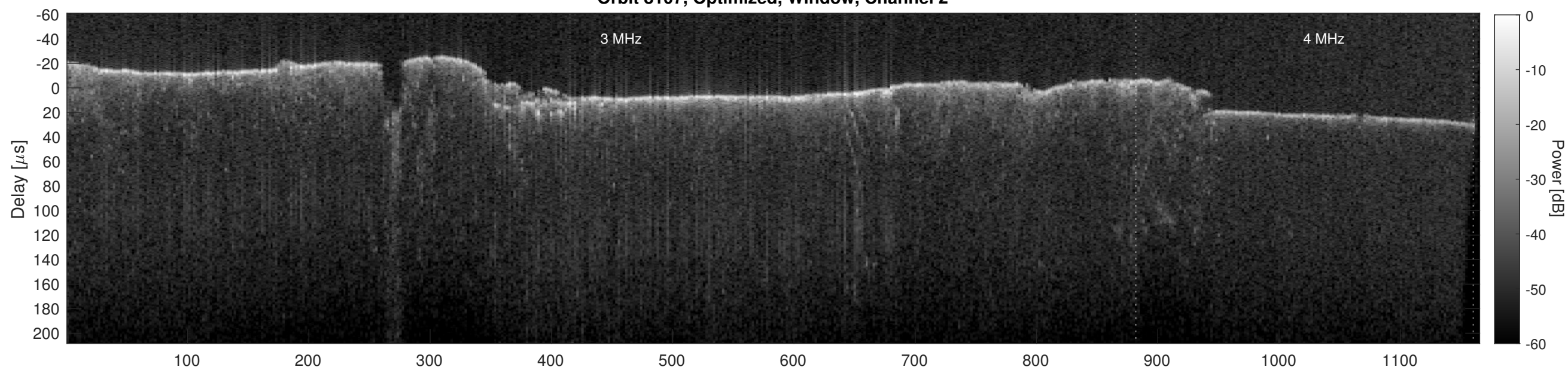
Orbit 8107, Cluttergram
