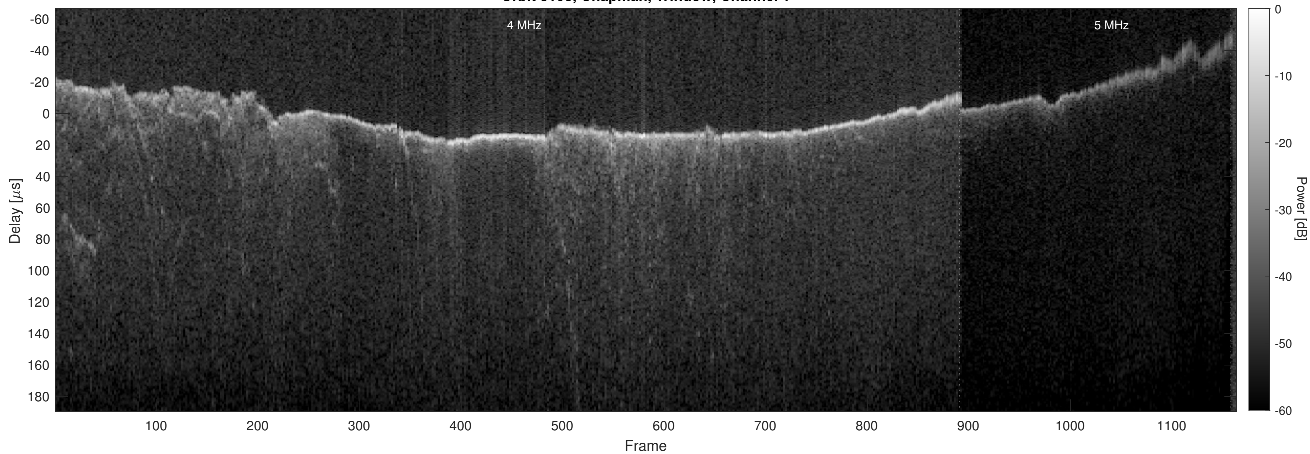
Orbit 8108, Chapman, Window, Channel 2
