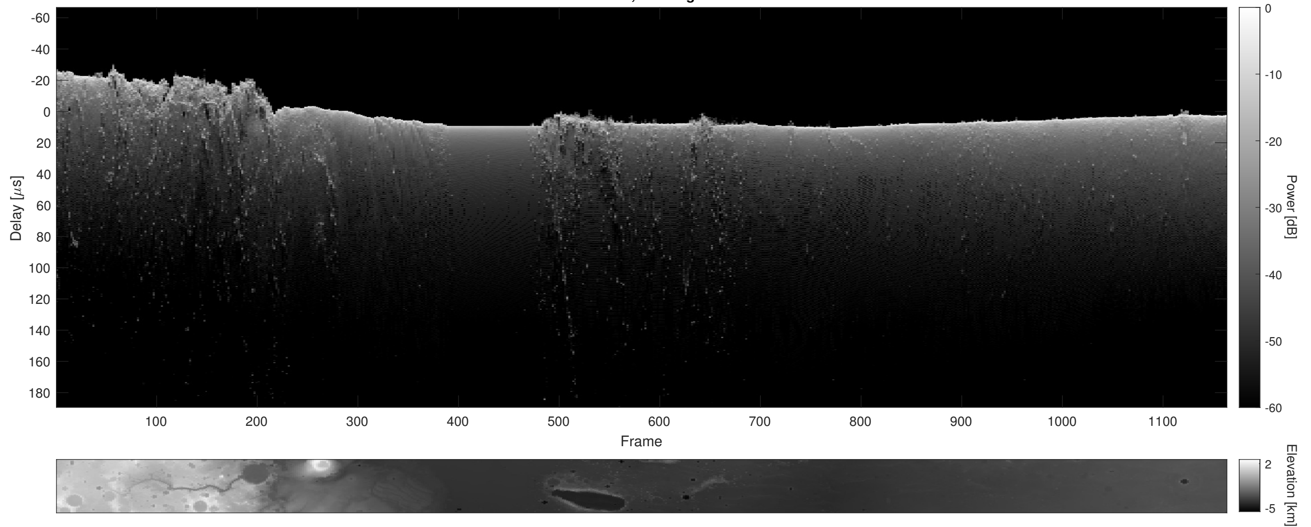
Orbit 8108, Cluttergram
