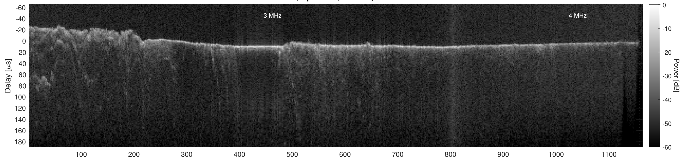
Orbit 8108, Cluttergram
