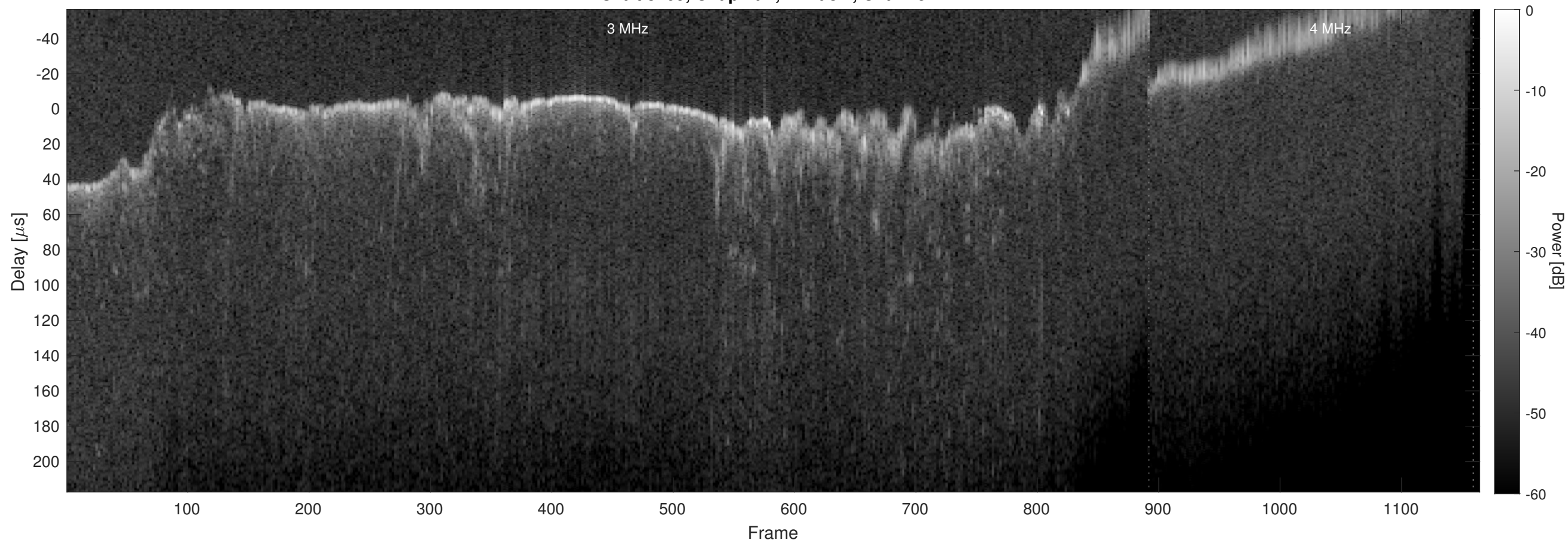
Orbit 8109, Chapman, Window, Channel 2
