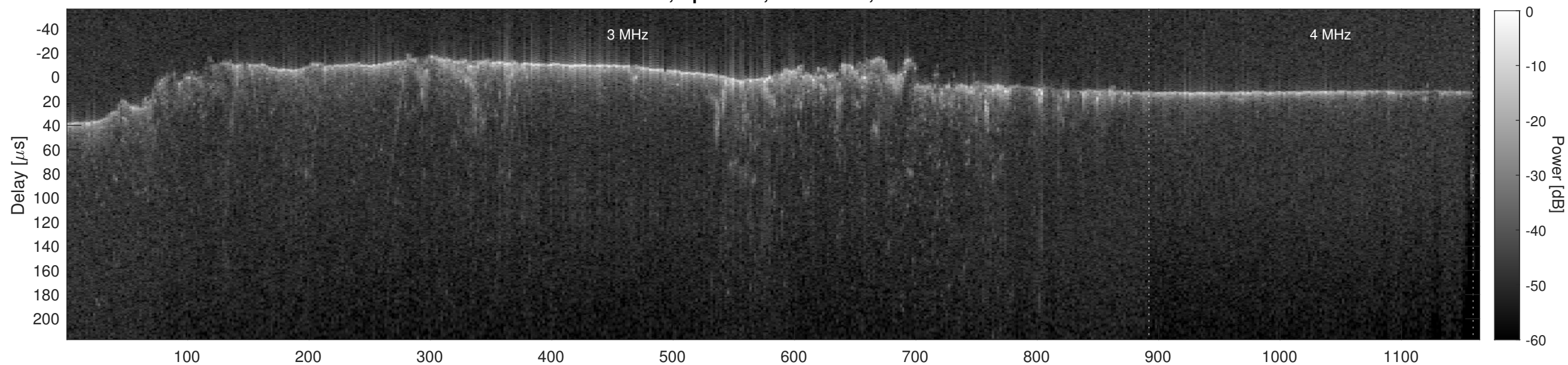
Orbit 8109, Cluttergram
