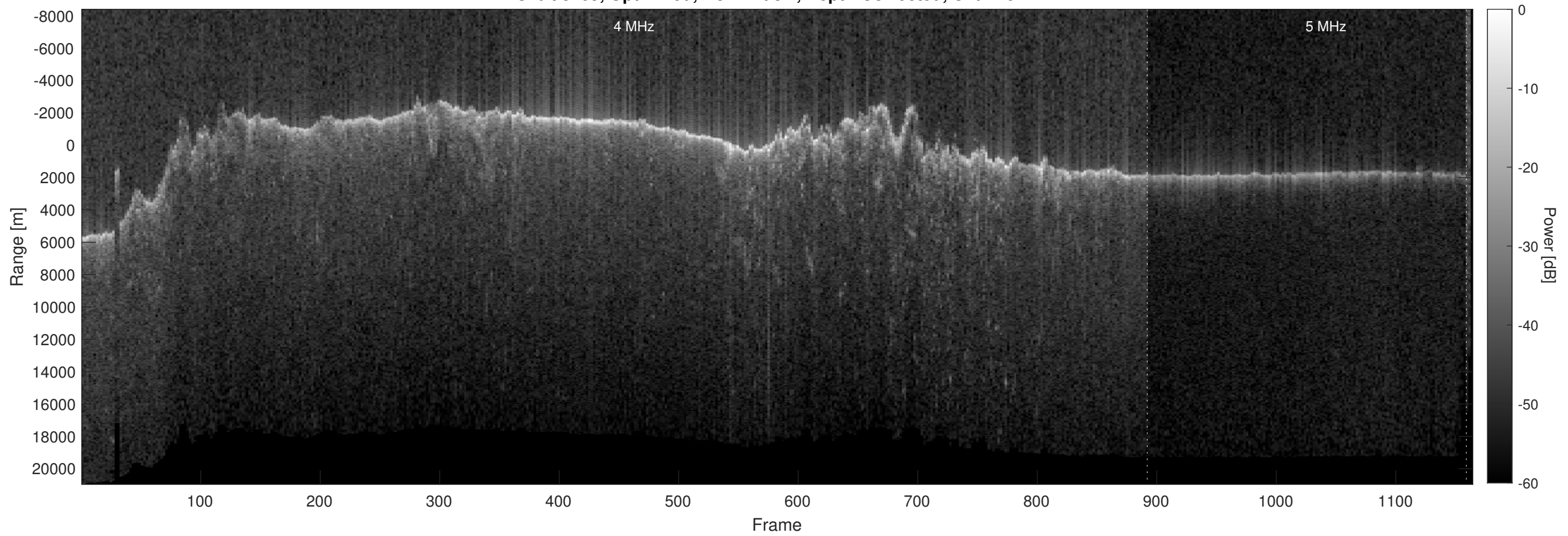
Orbit 8109, Optimized, No Window, Depth-Corrected, Channel 2
