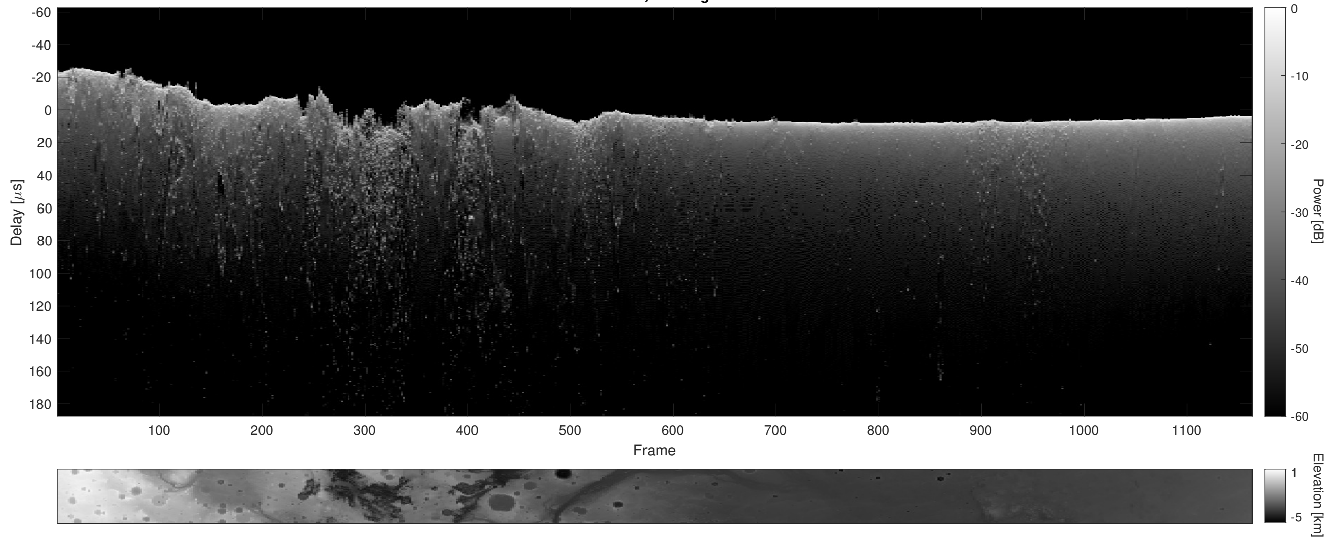
Orbit 8110, Cluttergram
