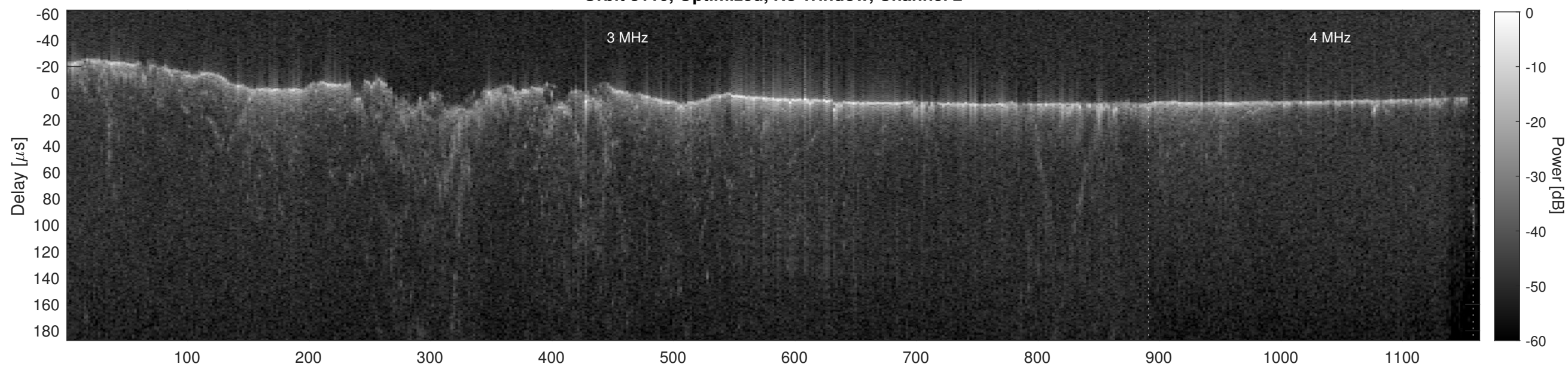
Orbit 8110, Cluttergram
