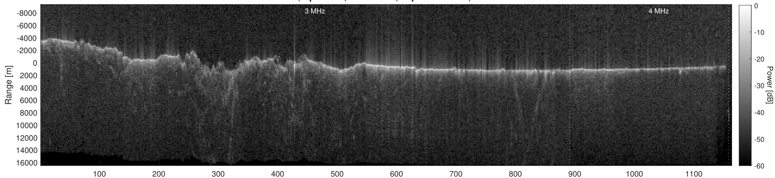
Orbit 8110, Depth-Corrected Cluttergram
