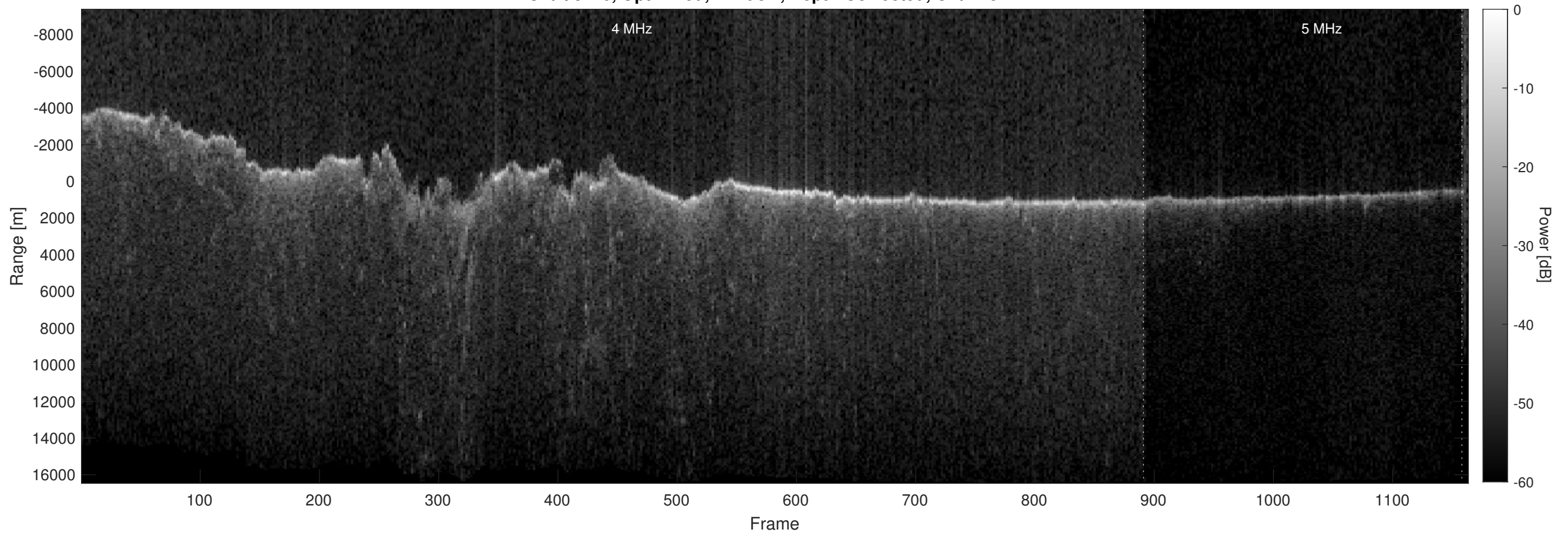
Orbit 8110, Optimized, Window, Depth-Corrected, Channel 2
