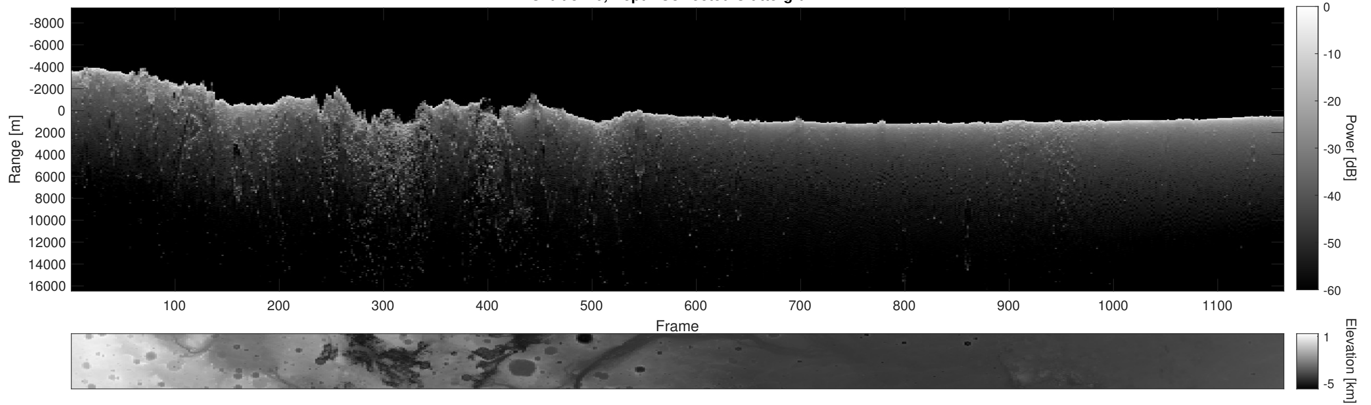
Orbit 8110, Depth-Corrected Cluttergram
