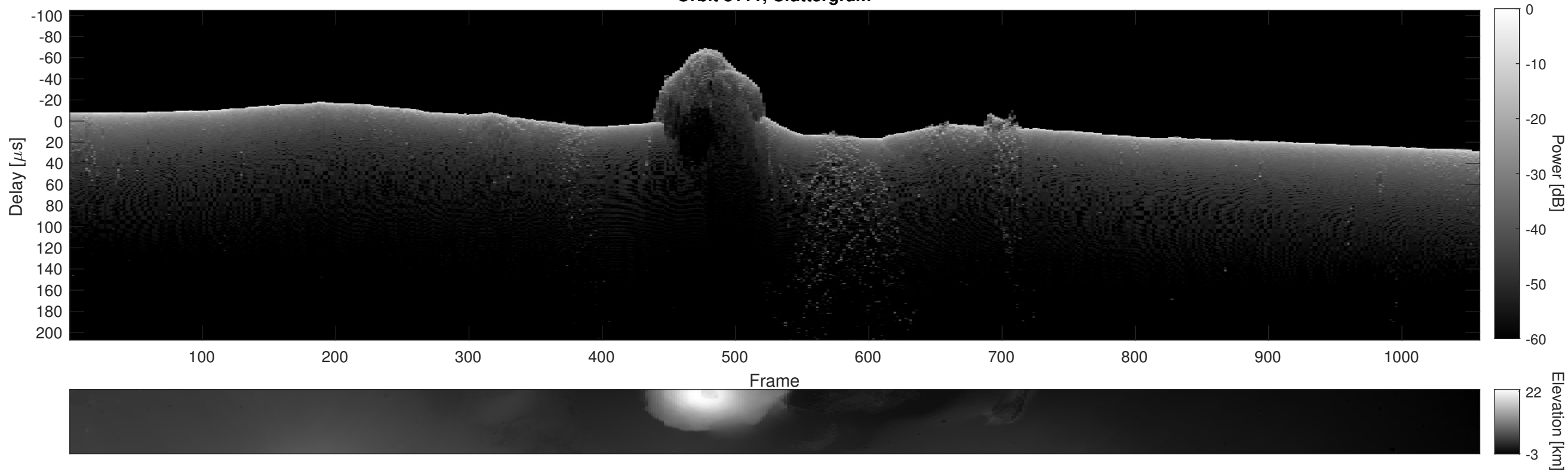
Orbit 8111, Cluttergram
