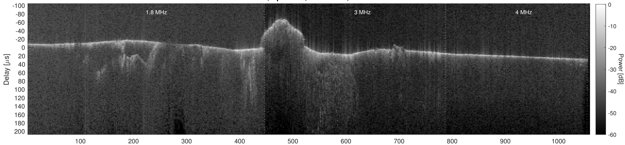
Orbit 8111, Cluttergram
