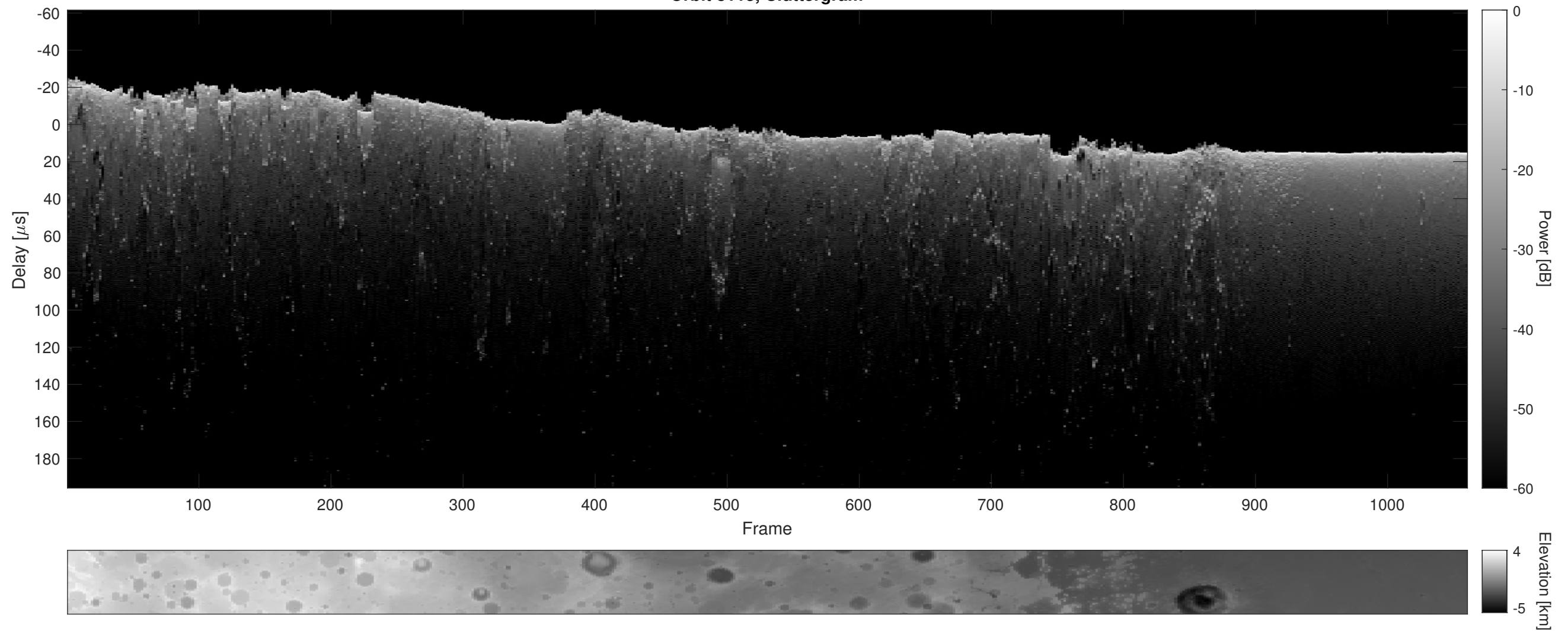
Orbit 8113, Cluttergram
