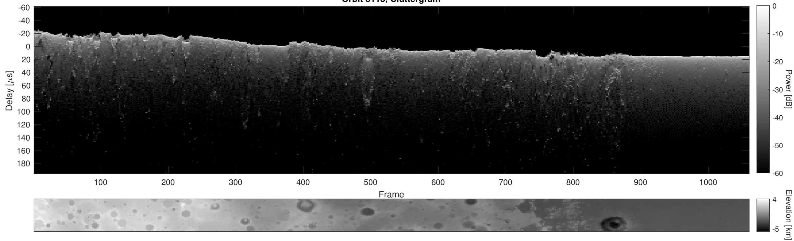
Orbit 8113, Cluttergram
