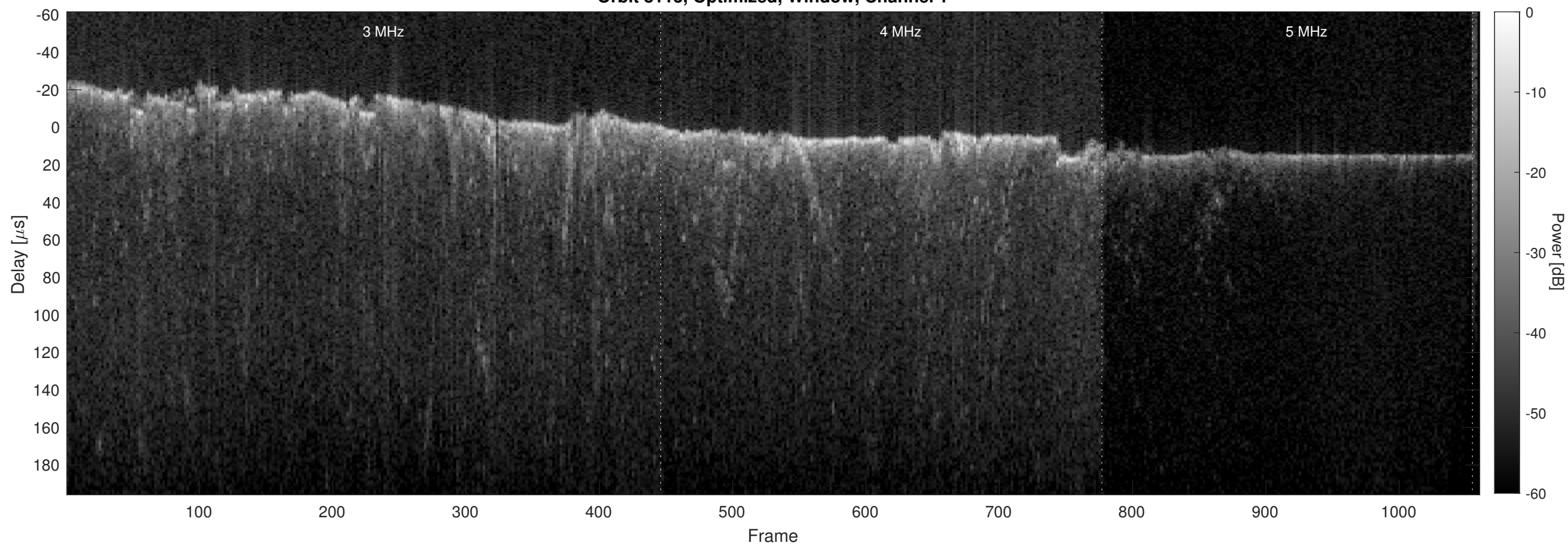
Orbit 8113, Optimized, Window, Channel 2
